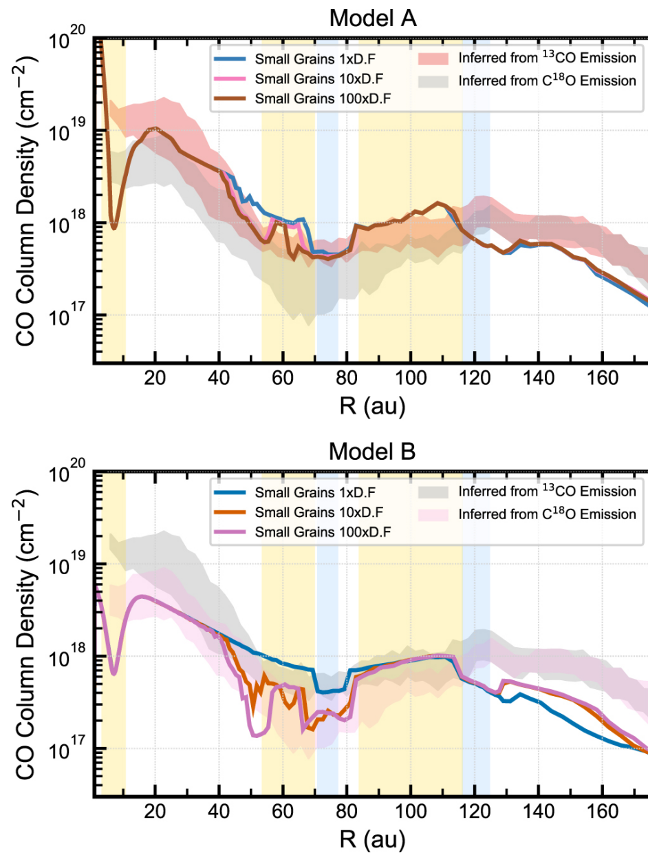
Figure 4. from Felipe Alarcón et al 2021 Astrophys. J. Suppl. 257 doi:10.3847/1538-4365/ac22ae https://dx.doi.org/10.3847/1538-4365/ac22ae © 2021. The American Astronomical Society. All rights reserved.
