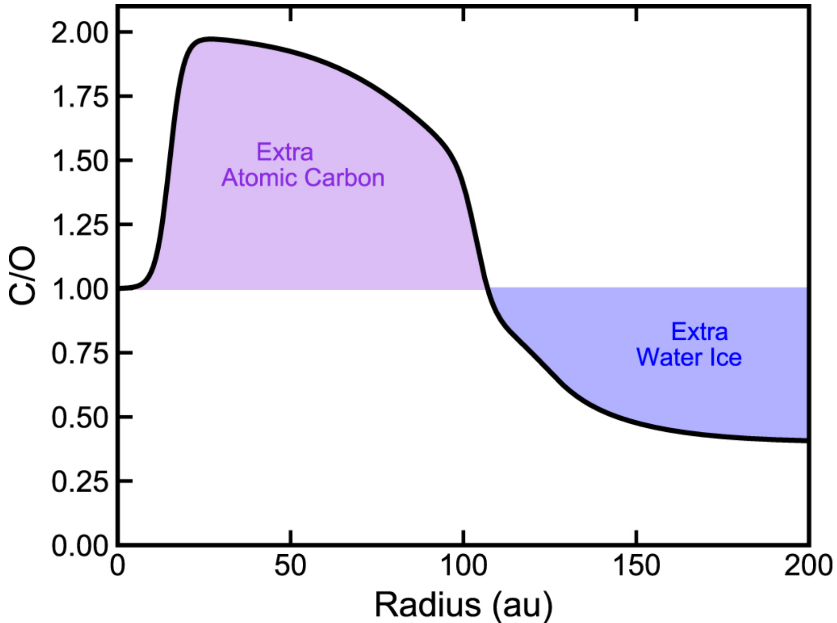
Figure 3. from Felipe Alarcón et al 2021 Astrophys. J. Suppl. 257 doi:10.3847/1538-4365/ac22ae https://dx.doi.org/10.3847/1538-4365/ac22ae © 2021. The American Astronomical Society. All rights reserved.
