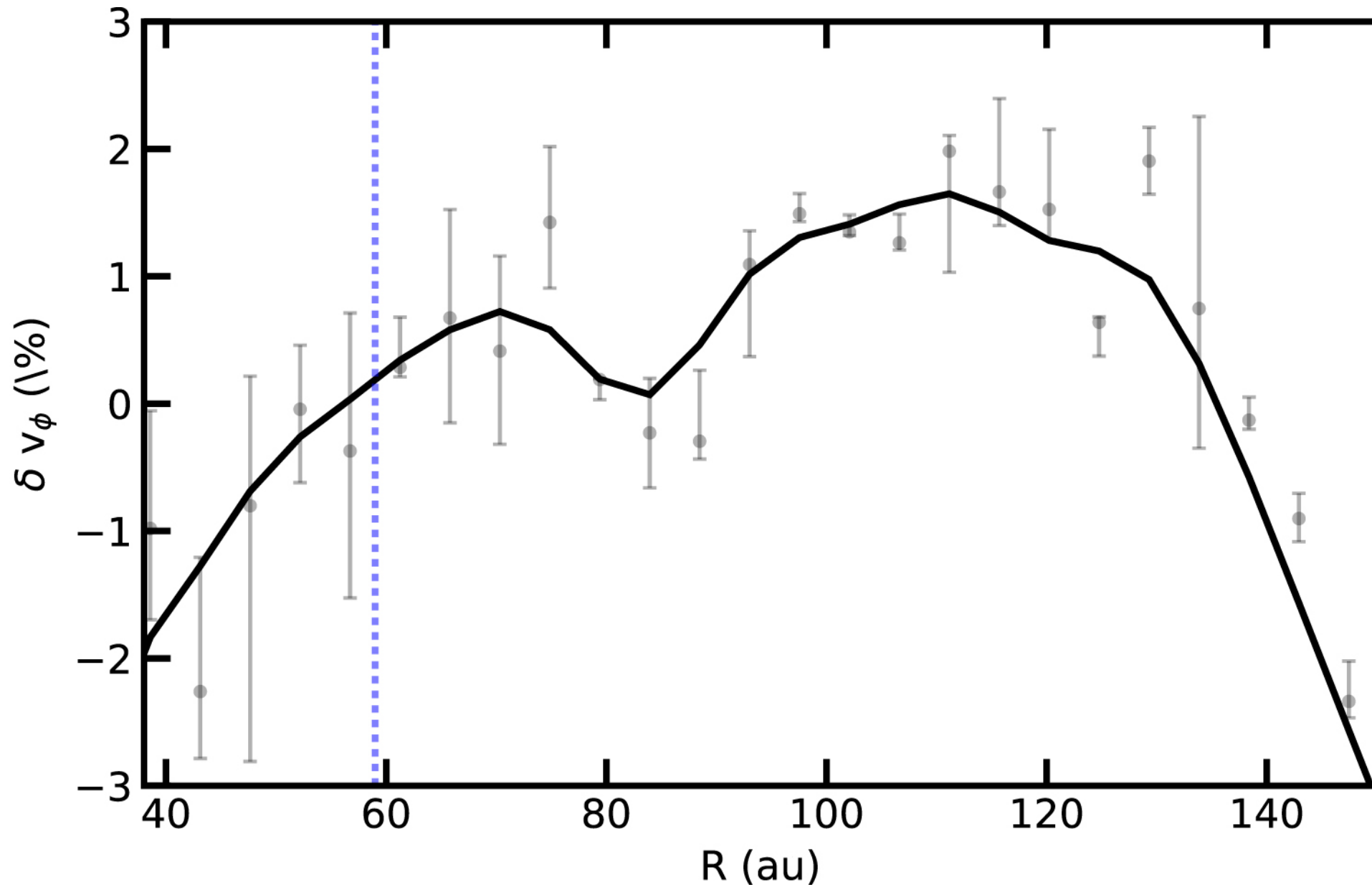
Figure 17. from Felipe Alarcón et al 2021 Astrophys. J. Suppl. 257 doi:10.3847/1538-4365/ac22ae https://dx.doi.org/10.3847/1538-4365/ac22ae © 2021. The American Astronomical Society. All rights reserved.
