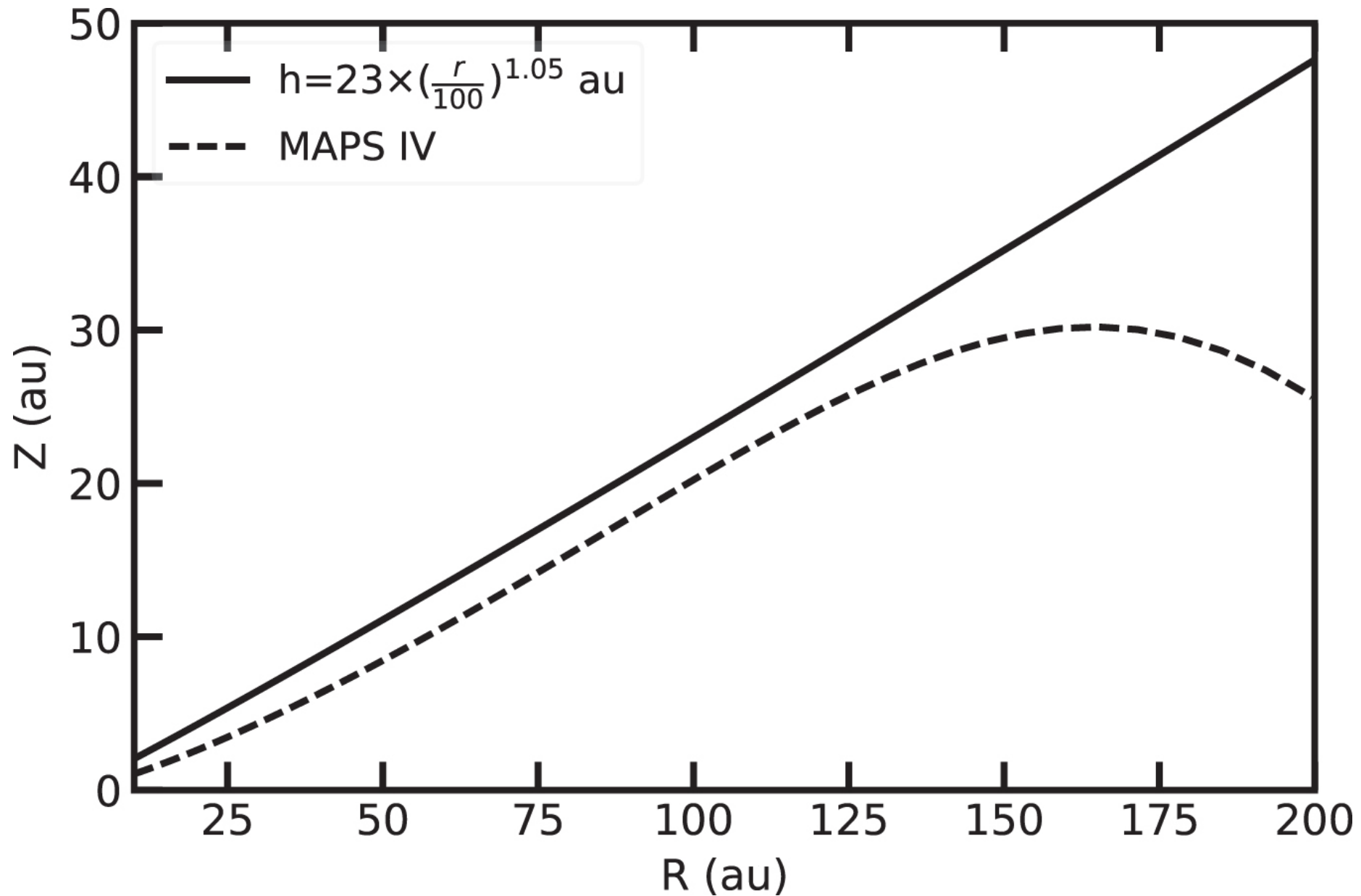
Figure 16. from Felipe Alarcón et al 2021 Astrophys. J. Suppl. 257 doi:10.3847/1538-4365/ac22ae https://dx.doi.org/10.3847/1538-4365/ac22ae © 2021. The American Astronomical Society. All rights reserved.
