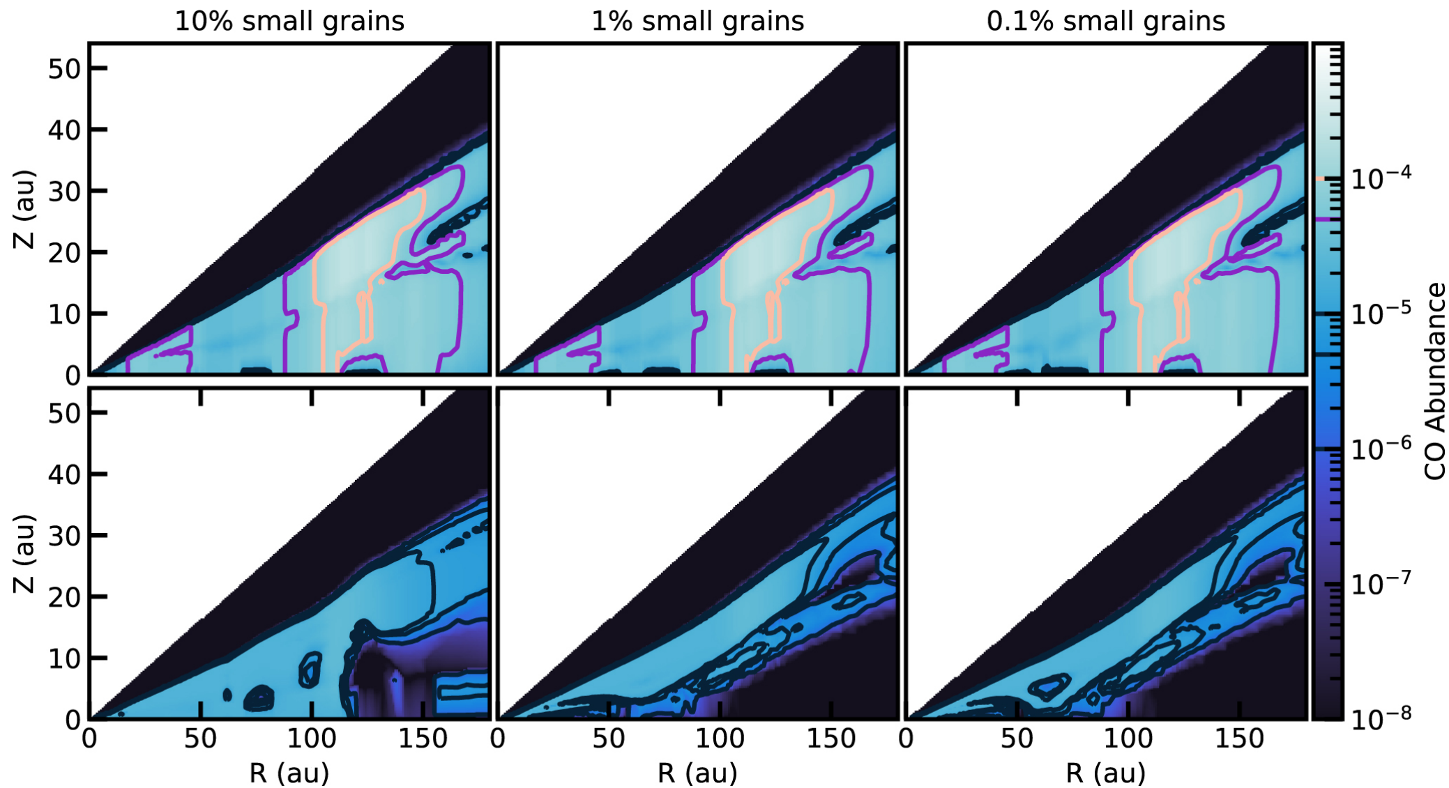
Figure 14. from Felipe Alarcón et al 2021 Astrophys. J. Suppl. 257 doi:10.3847/1538-4365/ac22ae https://dx.doi.org/10.3847/1538-4365/ac22ae © 2021. The American Astronomical Society. All rights reserved.
