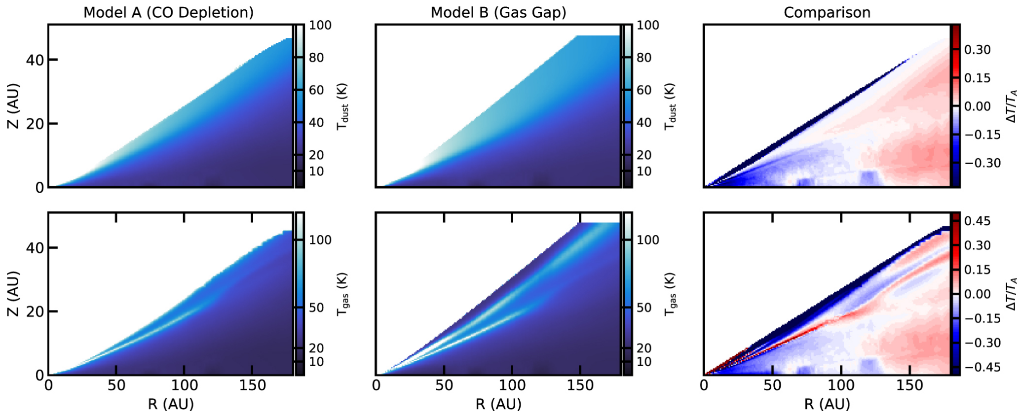
Figure 13. from Felipe Alarcón et al 2021 Astrophys. J. Suppl. 257 doi:10.3847/1538-4365/ac22ae https://dx.doi.org/10.3847/1538-4365/ac22ae © 2021. The American Astronomical Society. All rights reserved.
