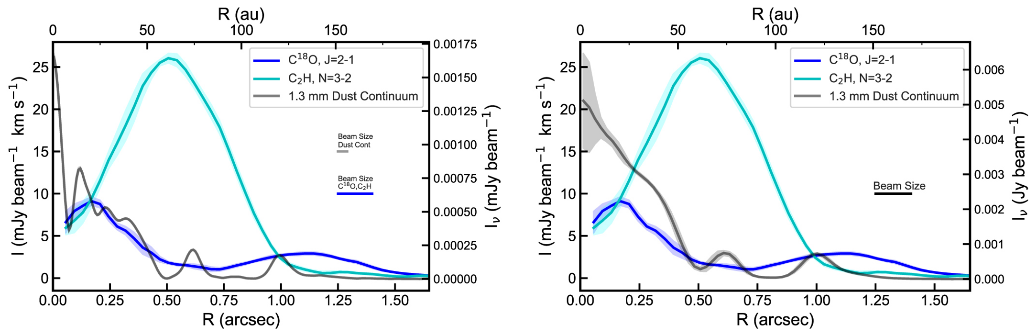
Figure 11. from Felipe Alarcón et al 2021 Astrophys. J. Suppl. 257 doi:10.3847/1538-4365/ac22ae https://dx.doi.org/10.3847/1538-4365/ac22ae © 2021. The American Astronomical Society. All rights reserved.
