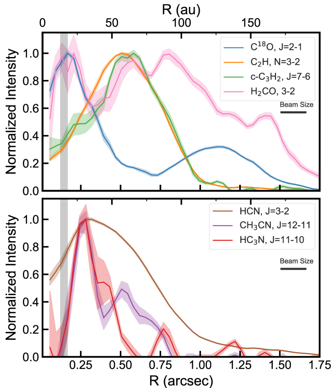
Figure 10. from Felipe Alarcón et al 2021 Astrophys. J. Suppl. 257 doi:10.3847/1538-4365/ac22ae https://dx.doi.org/10.3847/1538-4365/ac22ae © 2021. The American Astronomical Society. All rights reserved.
