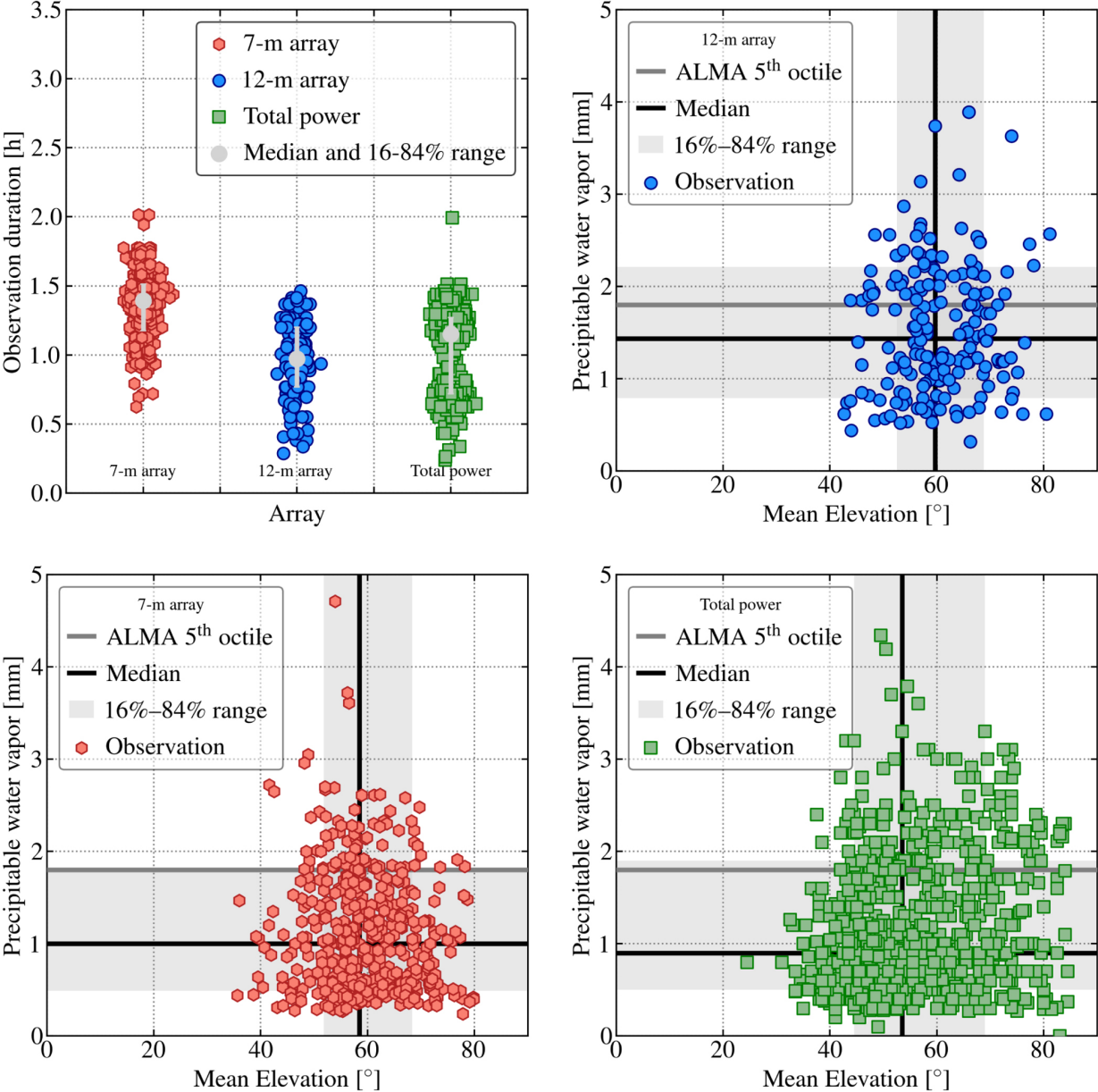
Figure 22. from Adam K. Leroy et al 2021 Astrophys. J. Suppl. 257 doi:10.3847/1538-4365/ac17f3 https://dx.doi.org/10.3847/1538-4365/ac17f3 © 2021. The American Astronomical Society. All rights reserved.
