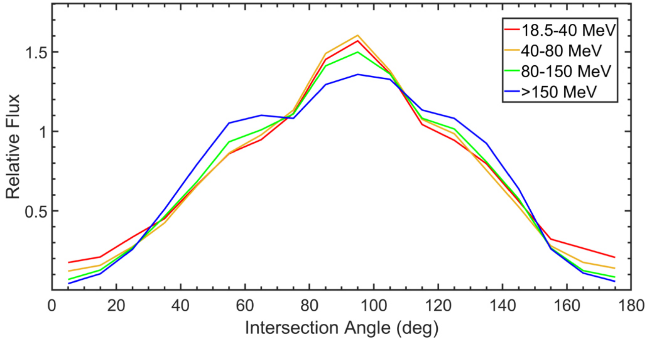
Figure 8. from Yuan You et al 2021 Astrophys. J. Suppl. 256 doi:10.3847/1538-4365/ac16db https://dx.doi.org/10.3847/1538-4365/ac16db © 2021. The American Astronomical Society. All rights reserved.
