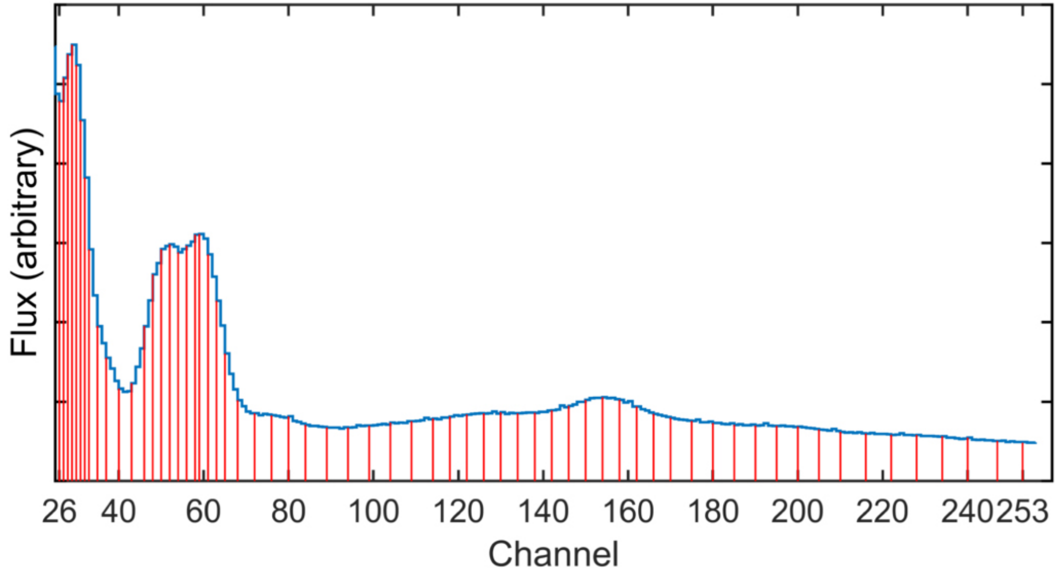
Figure 10. from Yuan You et al 2021 Astrophys. J. Suppl. 256 doi:10.3847/1538-4365/ac16db https://dx.doi.org/10.3847/1538-4365/ac16db © 2021. The American Astronomical Society. All rights reserved.
