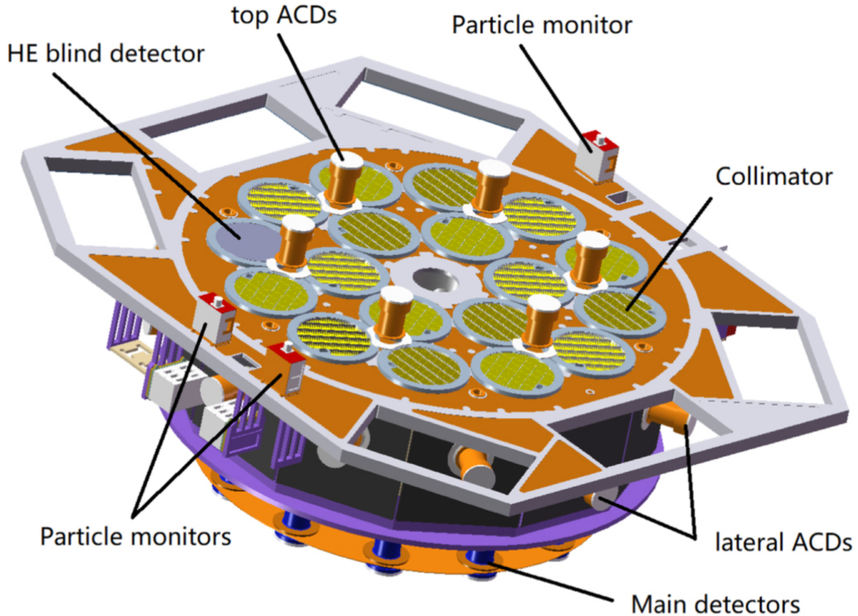
Figure 1. from Yuan You et al 2021 Astrophys. J. Suppl. 256 doi:10.3847/1538-4365/ac16db https://dx.doi.org/10.3847/1538-4365/ac16db © 2021. The American Astronomical Society. All rights reserved.
