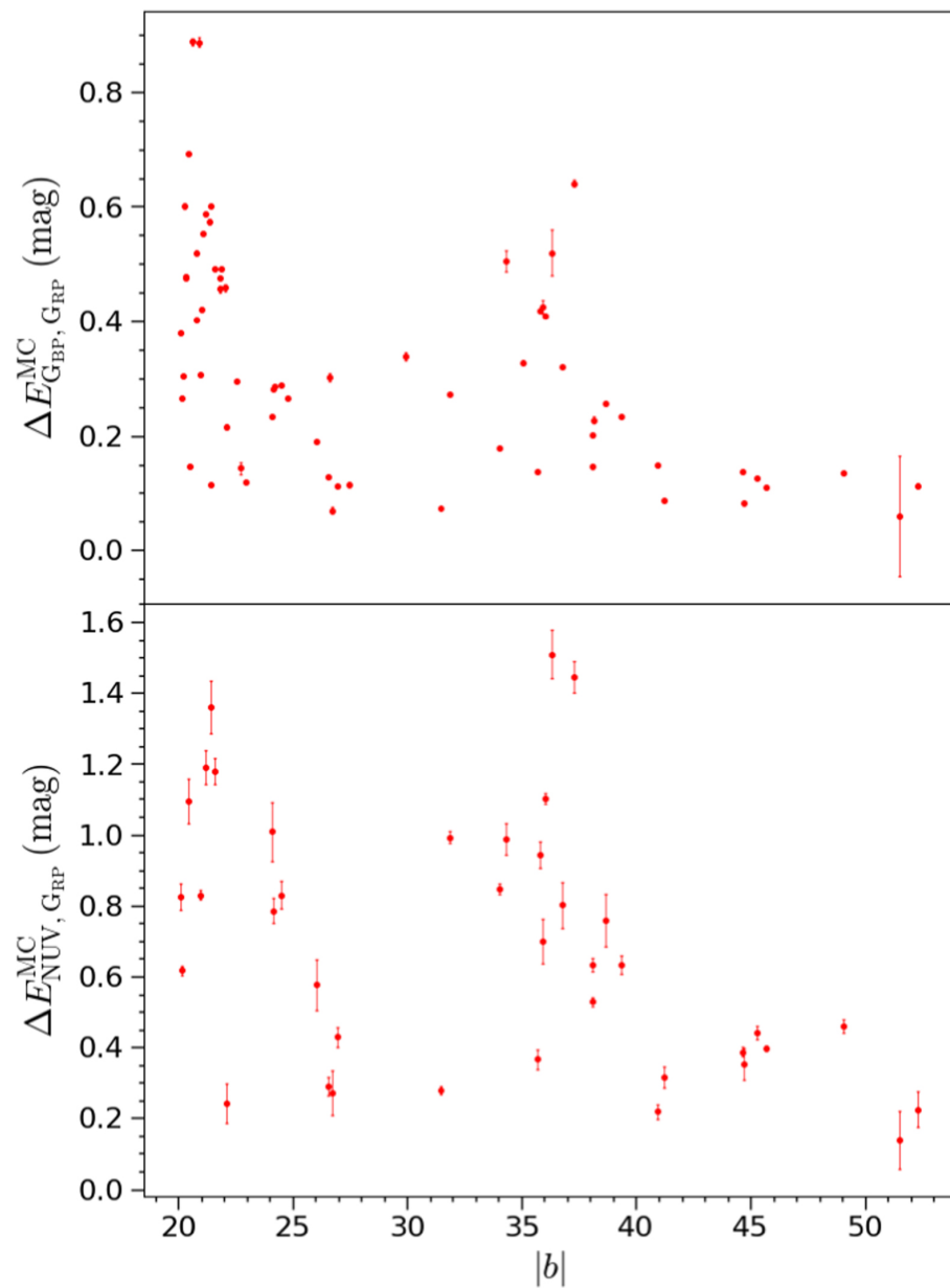
Figure 9. from Mingxu Sun et al 2021 Astrophys. J. Suppl. 256 doi:10.3847/1538-4365/ac1601 https://dx.doi.org/10.3847/1538-4365/ac1601 © 2021. The Author(s). Published by the American Astronomical Society.
