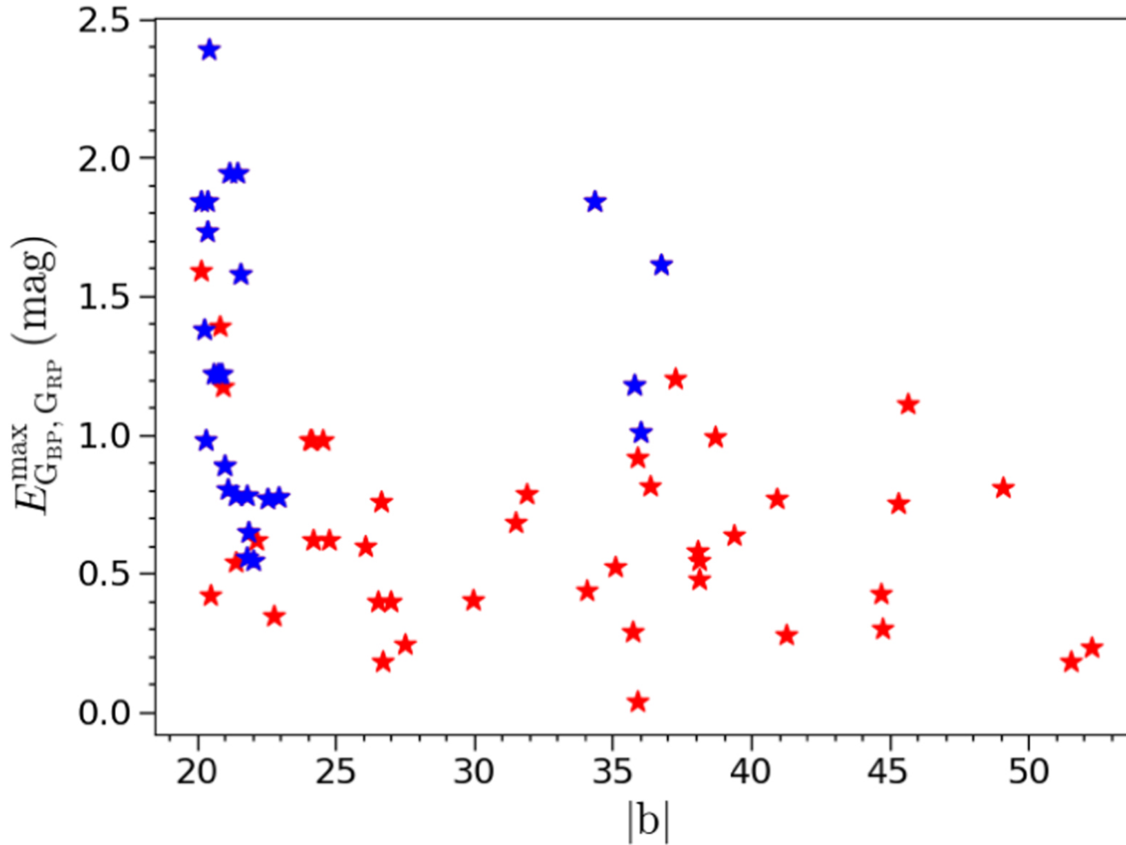
Figure 10. from Mingxu Sun et al 2021 Astrophys. J. Suppl. 256 doi:10.3847/1538-4365/ac1601 https://dx.doi.org/10.3847/1538-4365/ac1601 © 2021. The Author(s). Published by the American Astronomical Society.
