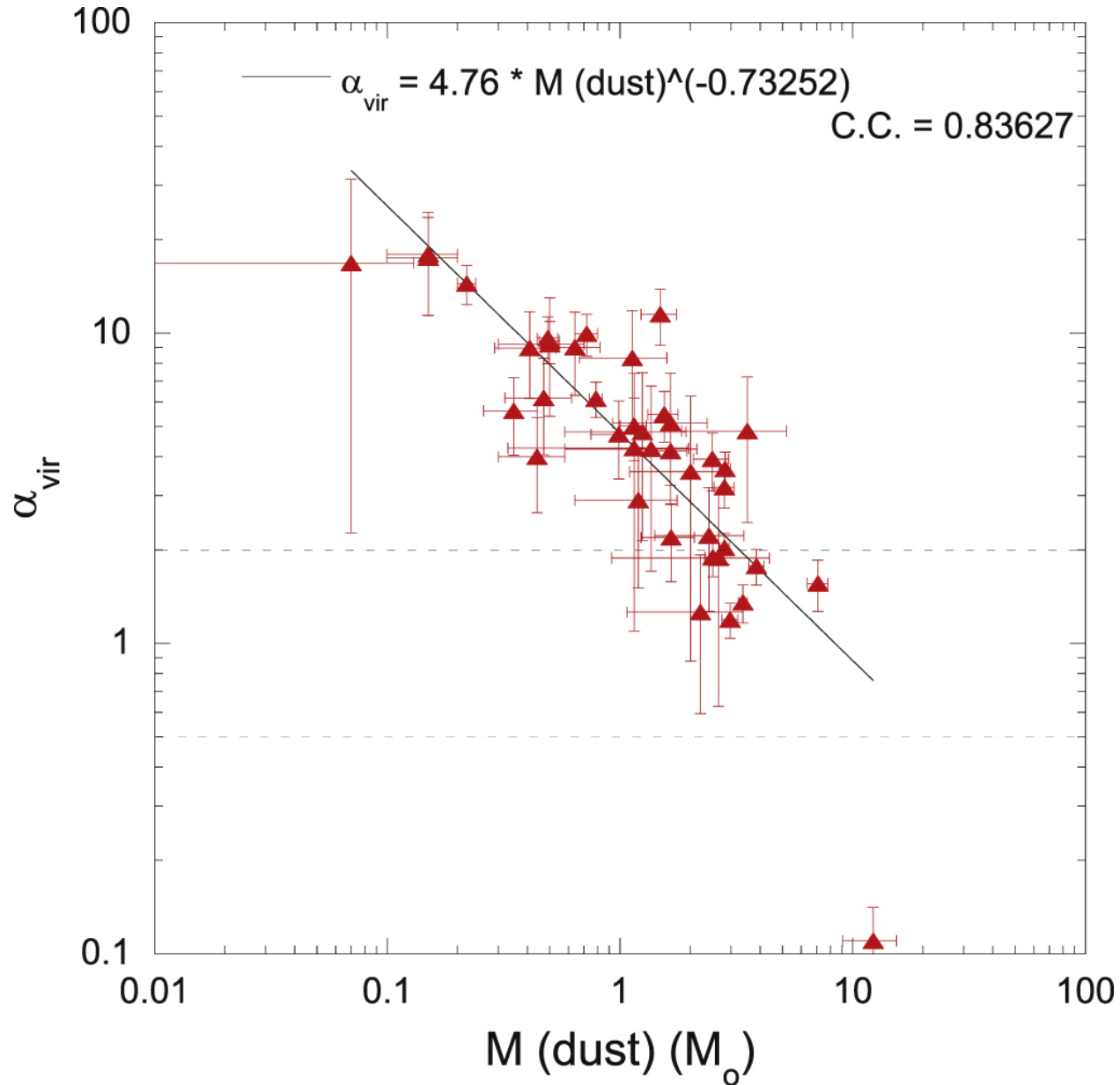
Figure 9. from Molecular Cloud Cores with High Deuterium Fractions: Nobeyama Mapping Survey null 2021 APJS 256 25 doi:10.3847/1538-4365/ac0978 https://dx.doi.org/10.3847/1538-4365/ac0978 © 2021. The American Astronomical Society. All rights reserved.
