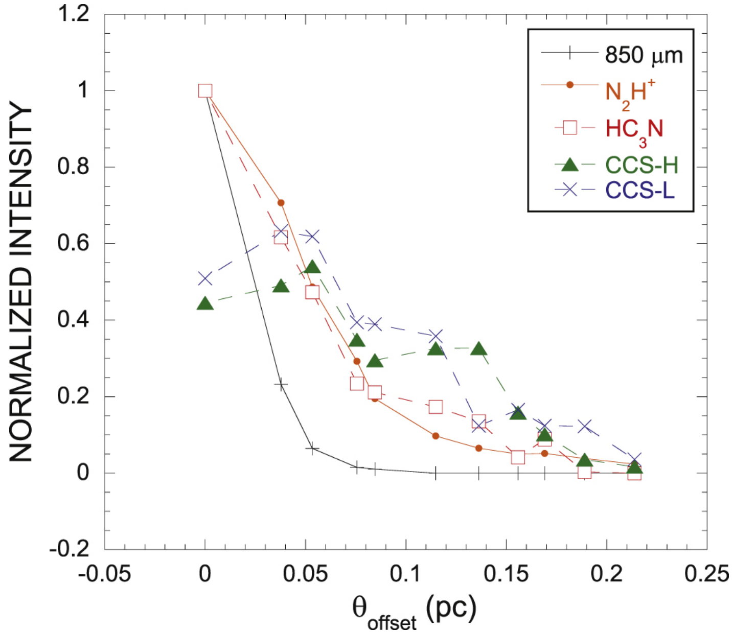
Figure 8. from Molecular Cloud Cores with High Deuterium Fractions: Nobeyama Mapping Survey null 2021 APJS 256 25 doi:10.3847/1538-4365/ac0978 https://dx.doi.org/10.3847/1538-4365/ac0978 © 2021. The American Astronomical Society. All rights reserved.
