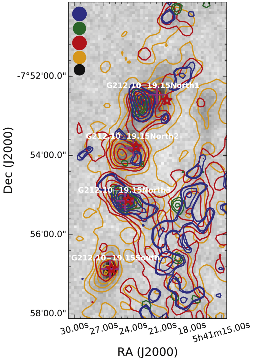
Figure 7. from Molecular Cloud Cores with High Deuterium Fractions: Nobeyama Mapping Survey null 2021 APJS 256 25 doi:10.3847/1538-4365/ac0978 https://dx.doi.org/10.3847/1538-4365/ac0978 © 2021. The American Astronomical Society. All rights reserved.
