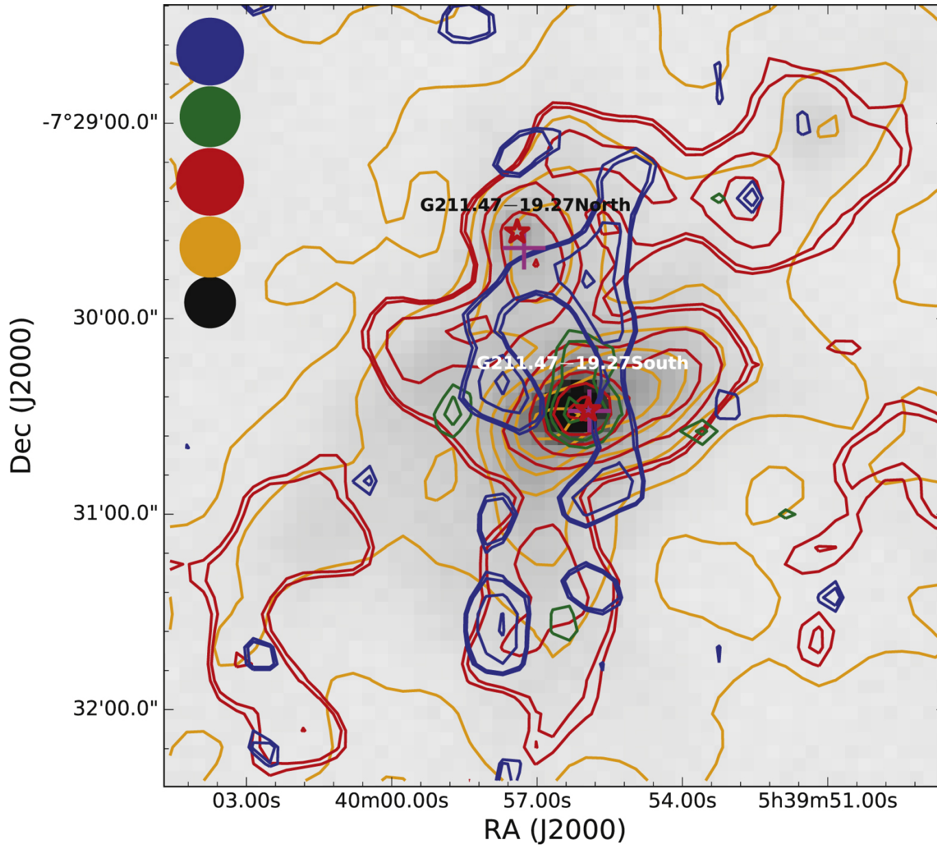
Figure 6. from Molecular Cloud Cores with High Deuterium Fractions: Nobeyama Mapping Survey null 2021 APJS 256 25 doi:10.3847/1538-4365/ac0978 https://dx.doi.org/10.3847/1538-4365/ac0978 © 2021. The American Astronomical Society. All rights reserved.
