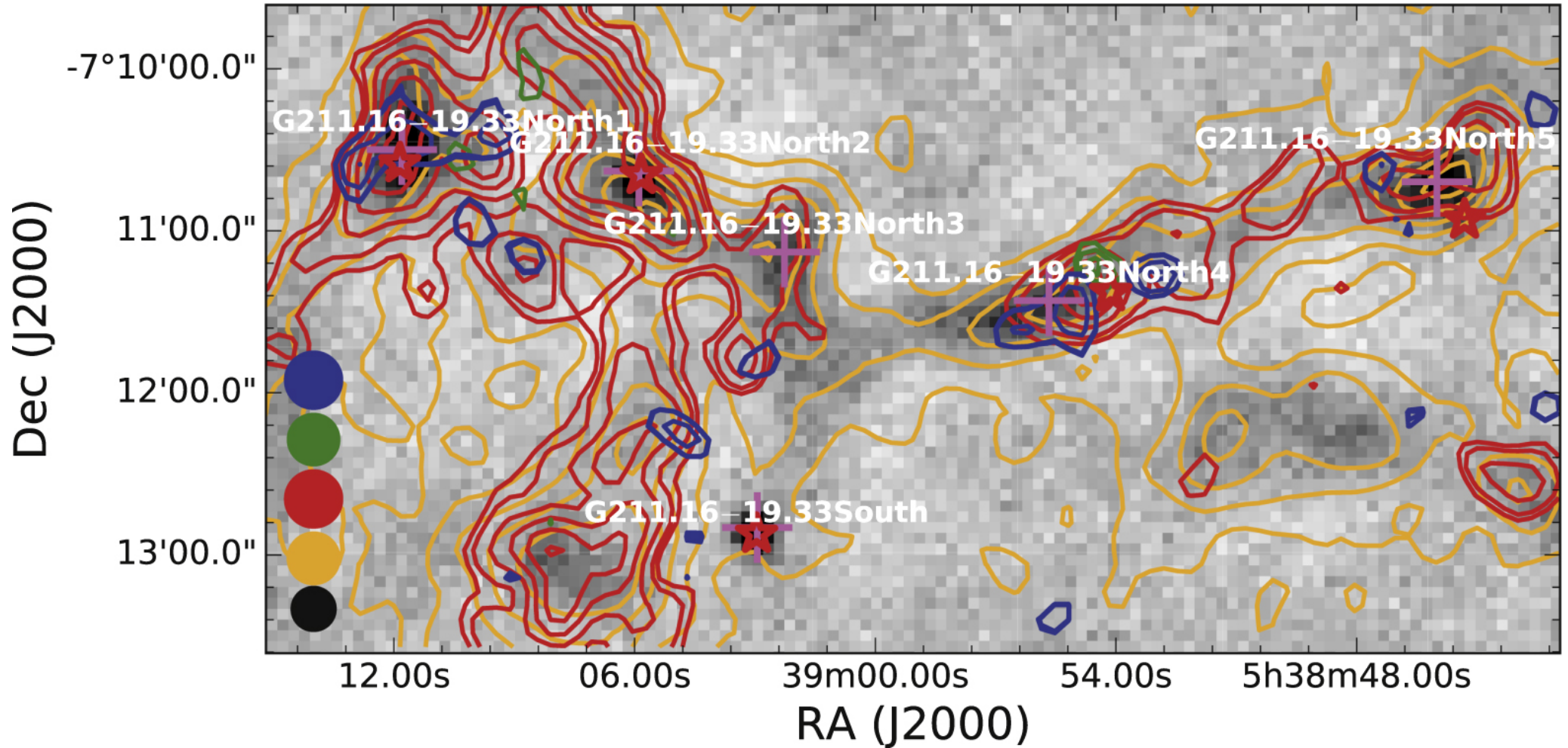
Figure 5. from Molecular Cloud Cores with High Deuterium Fractions: Nobeyama Mapping Survey null 2021 APJS 256 25 doi:10.3847/1538-4365/ac0978 https://dx.doi.org/10.3847/1538-4365/ac0978 © 2021. The American Astronomical Society. All rights reserved.
