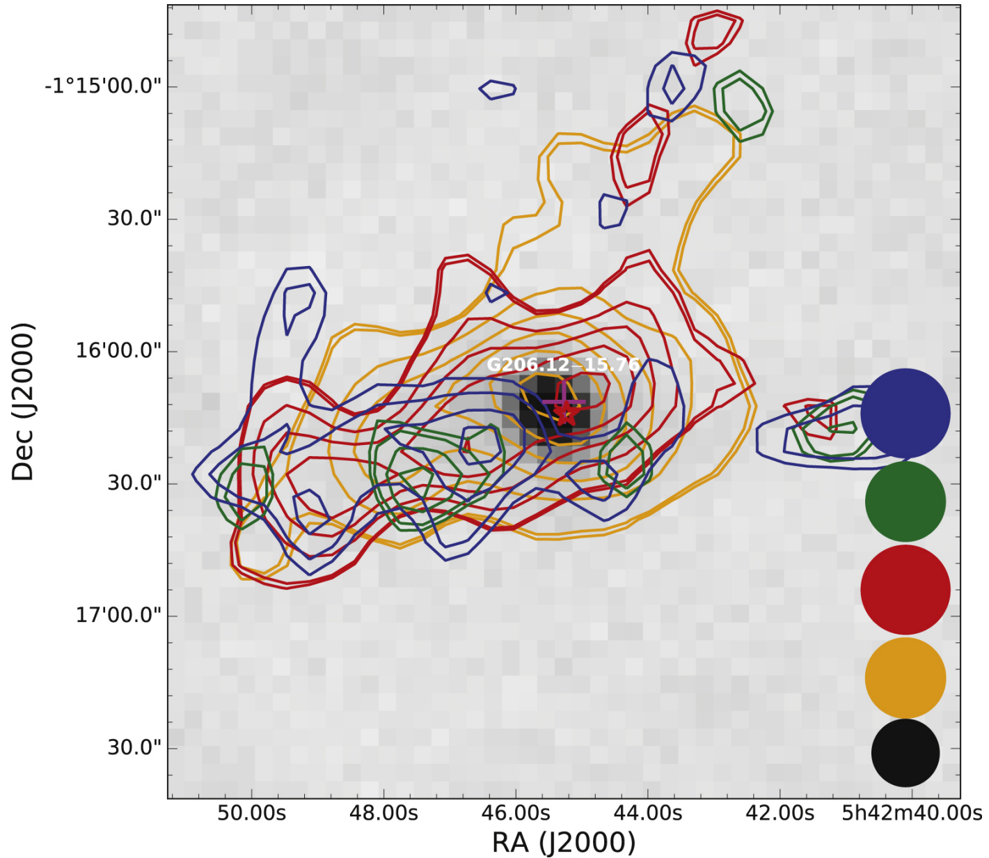
Figure 2. from Molecular Cloud Cores with High Deuterium Fractions: Nobeyama Mapping Survey null 2021 APJS 256 25 doi:10.3847/1538-4365/ac0978 https://dx.doi.org/10.3847/1538-4365/ac0978 © 2021. The American Astronomical Society. All rights reserved.
