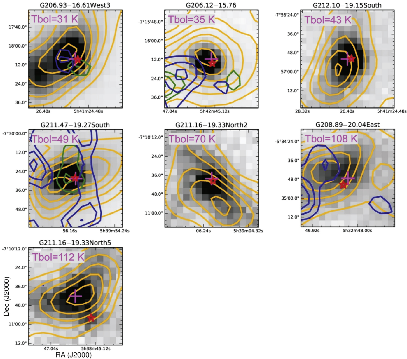
Figure 16. from Molecular Cloud Cores with High Deuterium Fractions: Nobeyama Mapping Survey null 2021 APJS 256 25 doi:10.3847/1538-4365/ac0978 https://dx.doi.org/10.3847/1538-4365/ac0978 © 2021. The American Astronomical Society. All rights reserved.
