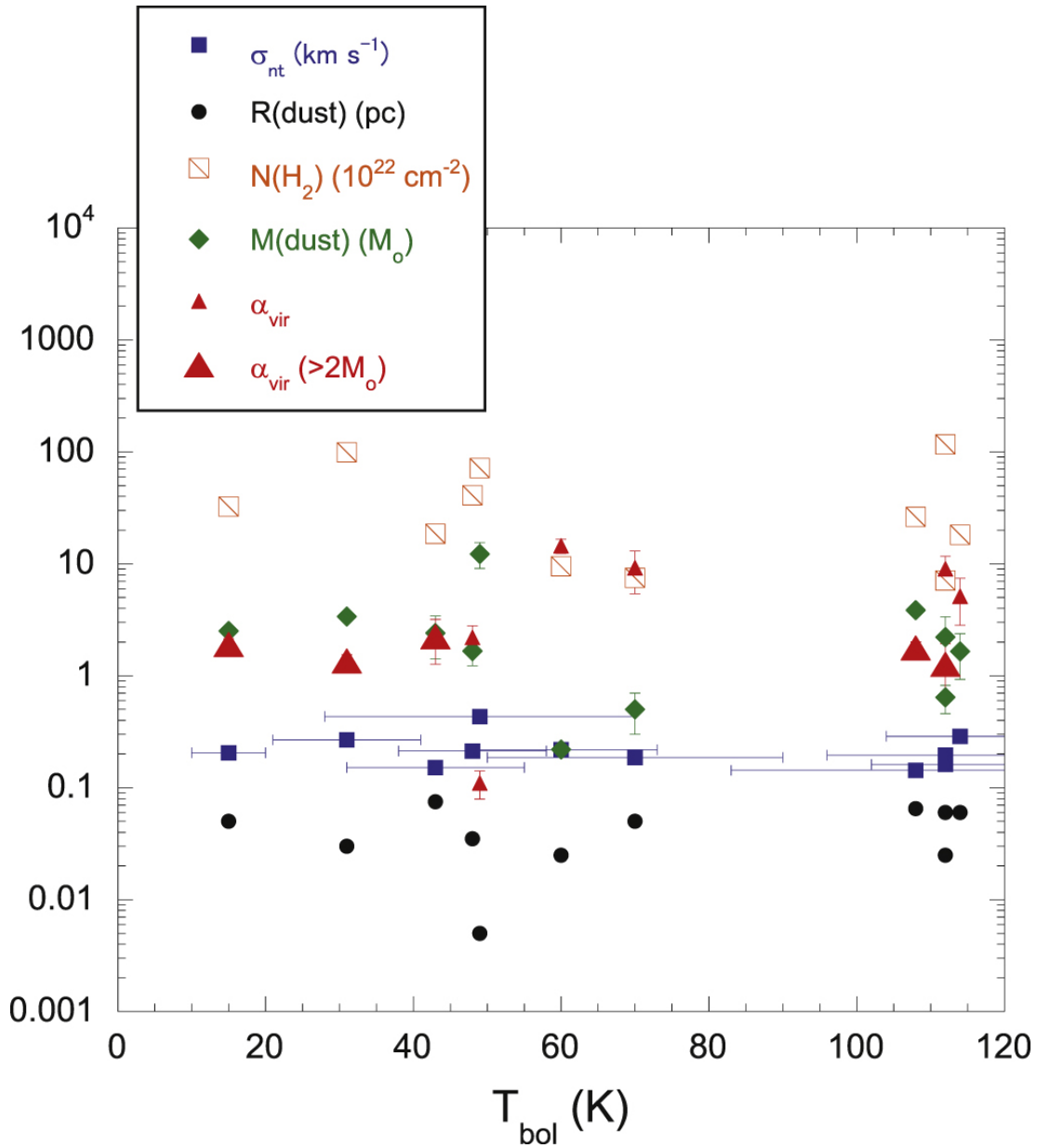
Figure 15. from Molecular Cloud Cores with High Deuterium Fractions: Nobeyama Mapping Survey null 2021 APJS 256 25 doi:10.3847/1538-4365/ac0978 https://dx.doi.org/10.3847/1538-4365/ac0978 © 2021. The American Astronomical Society. All rights reserved.
