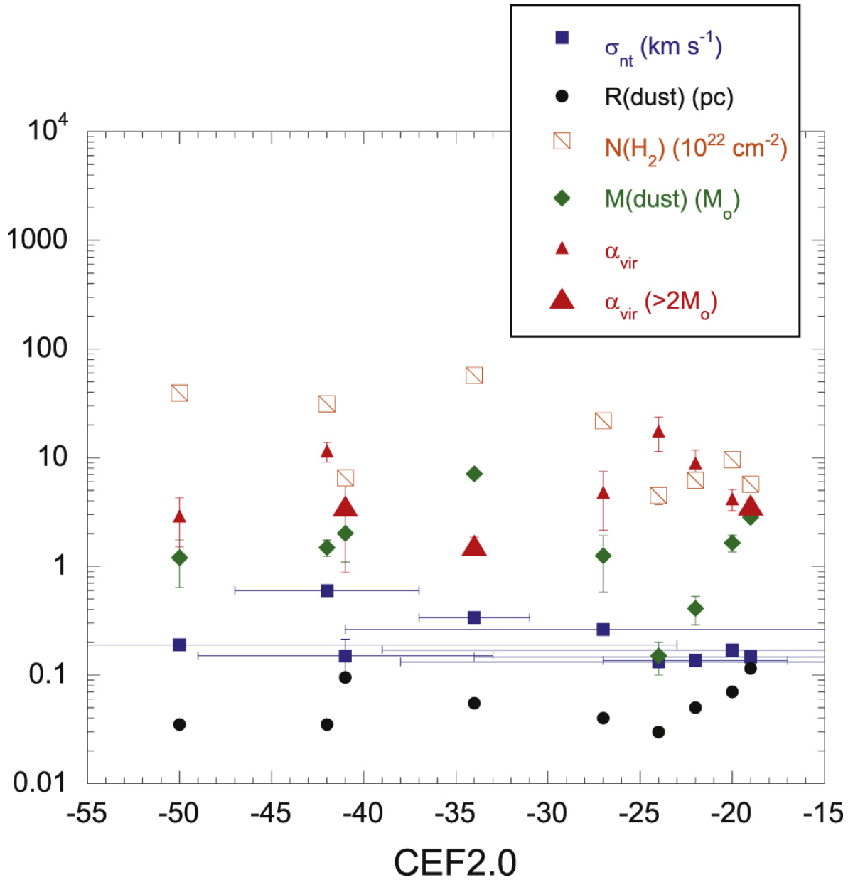
Figure 14. from Molecular Cloud Cores with High Deuterium Fractions: Nobeyama Mapping Survey null 2021 APJS 256 25 doi:10.3847/1538-4365/ac0978 https://dx.doi.org/10.3847/1538-4365/ac0978 © 2021. The American Astronomical Society. All rights reserved.
