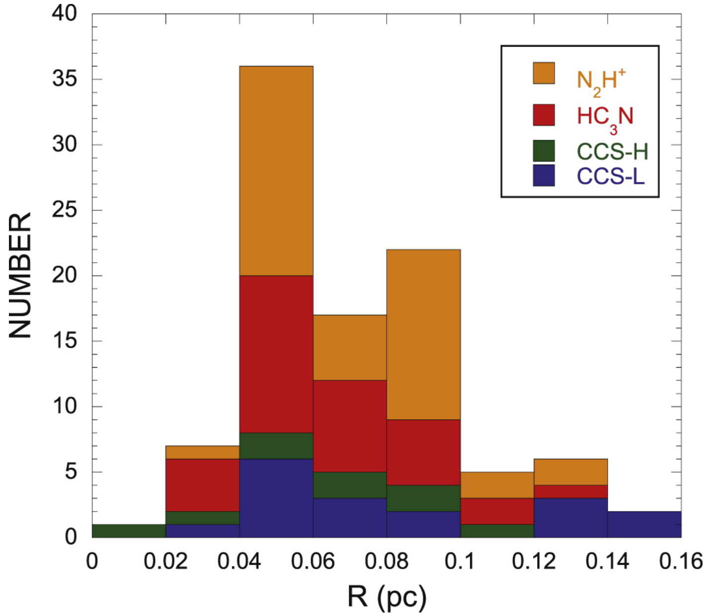
Figure 11. from Molecular Cloud Cores with High Deuterium Fractions: Nobeyama Mapping Survey null 2021 APJS 256 25 doi:10.3847/1538-4365/ac0978 https://dx.doi.org/10.3847/1538-4365/ac0978 © 2021. The American Astronomical Society. All rights reserved.
