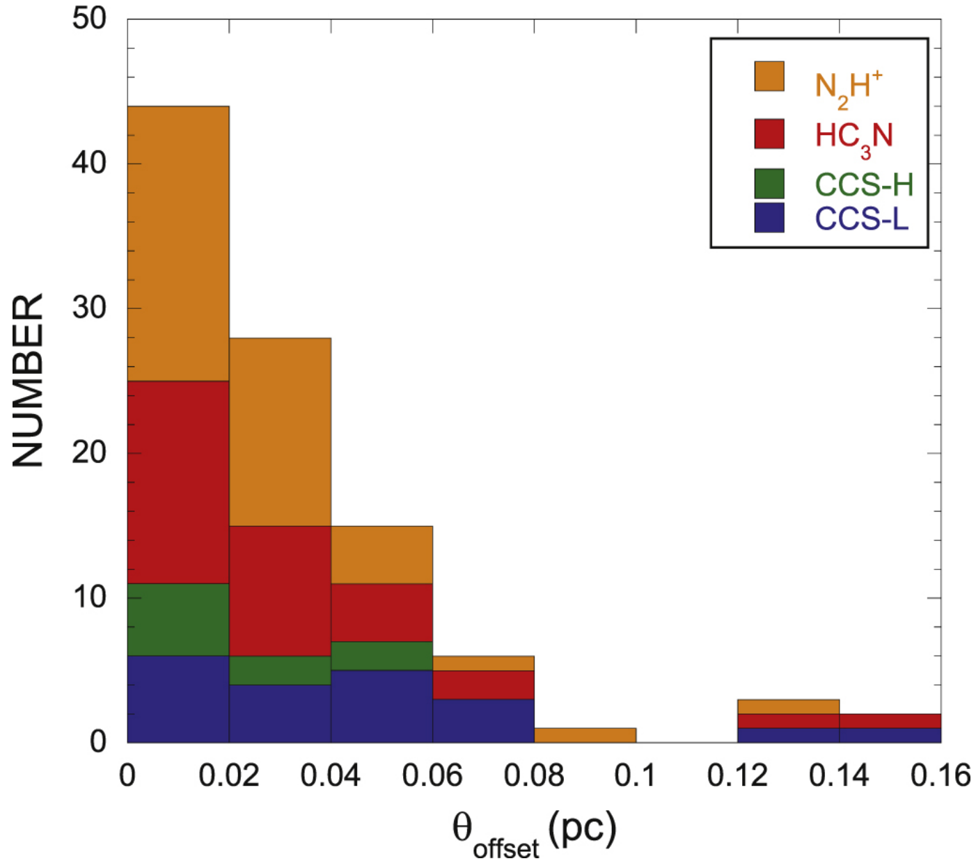
Figure 10. from Molecular Cloud Cores with High Deuterium Fractions: Nobeyama Mapping Survey null 2021 APJS 256 25 doi:10.3847/1538-4365/ac0978 https://dx.doi.org/10.3847/1538-4365/ac0978 © 2021. The American Astronomical Society. All rights reserved.
