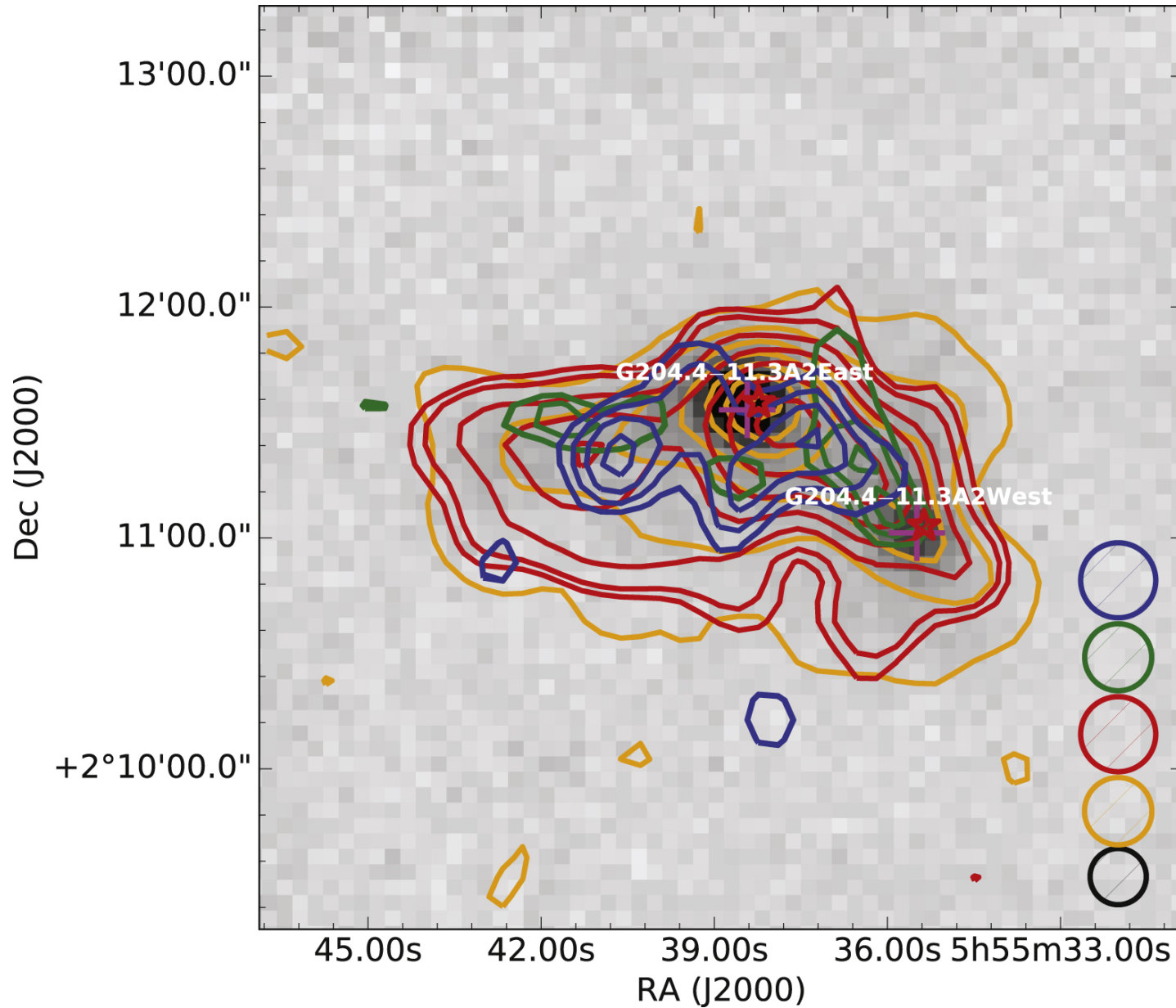
Figure 1. from Molecular Cloud Cores with High Deuterium Fractions: Nobeyama Mapping Survey null 2021 APJS 256 25 doi:10.3847/1538-4365/ac0978 https://dx.doi.org/10.3847/1538-4365/ac0978 © 2021. The American Astronomical Society. All rights reserved.
