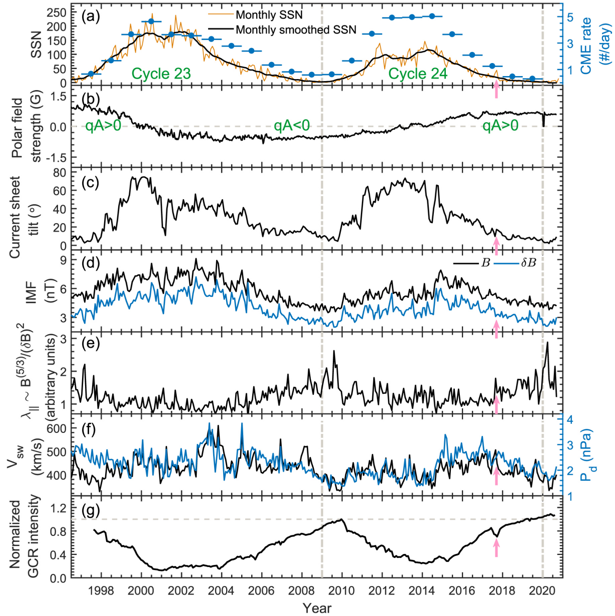
Figure 7. from Variations of the Galactic Cosmic Rays in the Recent Solar Cycles null 2021 APJS 254 37 doi:10.3847/1538-4365/abf936 https://dx.doi.org/10.3847/1538-4365/abf936 © 2021. The American Astronomical Society. All rights reserved.
