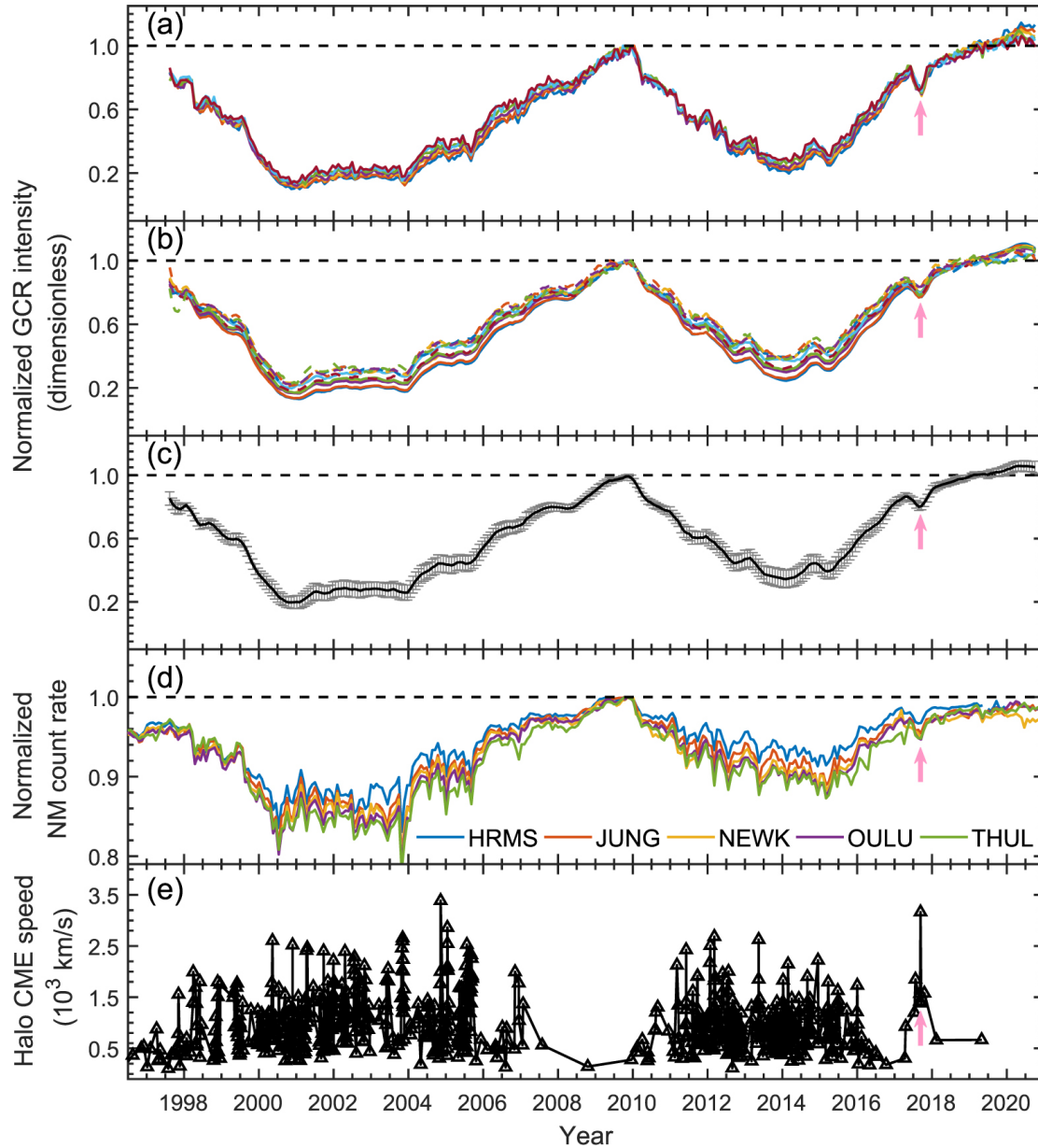
Figure 4. from Variations of the Galactic Cosmic Rays in the Recent Solar Cycles null 2021 APJS 254 37 doi:10.3847/1538-4365/abf936 https://dx.doi.org/10.3847/1538-4365/abf936 © 2021. The American Astronomical Society. All rights reserved.
