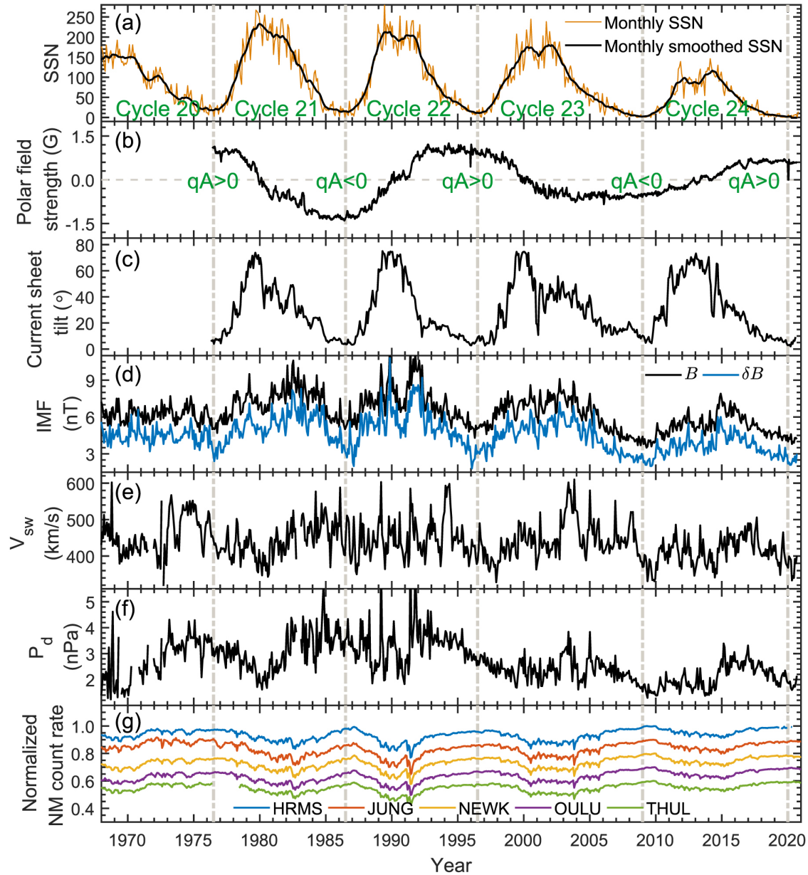
Figure 2. from Variations of the Galactic Cosmic Rays in the Recent Solar Cycles null 2021 APJS 254 37 doi:10.3847/1538-4365/abf936 https://dx.doi.org/10.3847/1538-4365/abf936 © 2021. The American Astronomical Society. All rights reserved.
