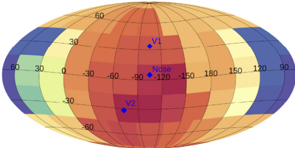
Figure 9. from A Three-dimensional Map of the Heliosphere from IBEX null 2021 APJS 254 40 doi:10.3847/1538-4365/abf658 https://dx.doi.org/10.3847/1538-4365/abf658 © 2021. The American Astronomical Society. All rights reserved.
