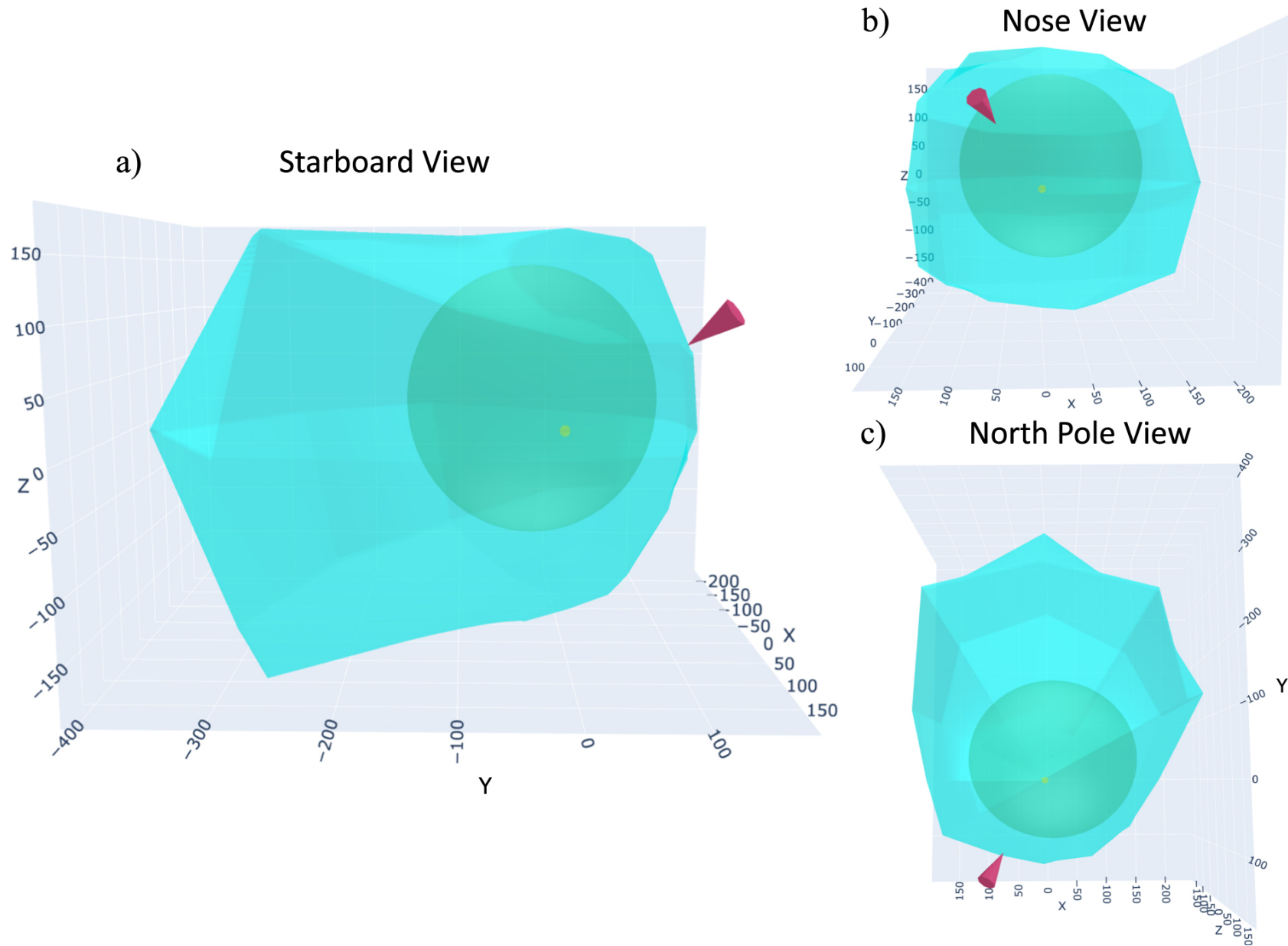
Figure 7. from A Three-dimensional Map of the Heliosphere from IBEX null 2021 APJS 254 40 doi:10.3847/1538-4365/abf658 https://dx.doi.org/10.3847/1538-4365/abf658 © 2021. The American Astronomical Society. All rights reserved.
