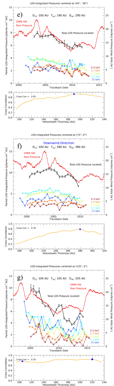
Figure 5. from A Three-dimensional Map of the Heliosphere from IBEX null 2021 APJS 254 40 doi:10.3847/1538-4365/abf658 https://dx.doi.org/10.3847/1538-4365/abf658 © 2021. The American Astronomical Society. All rights reserved.
