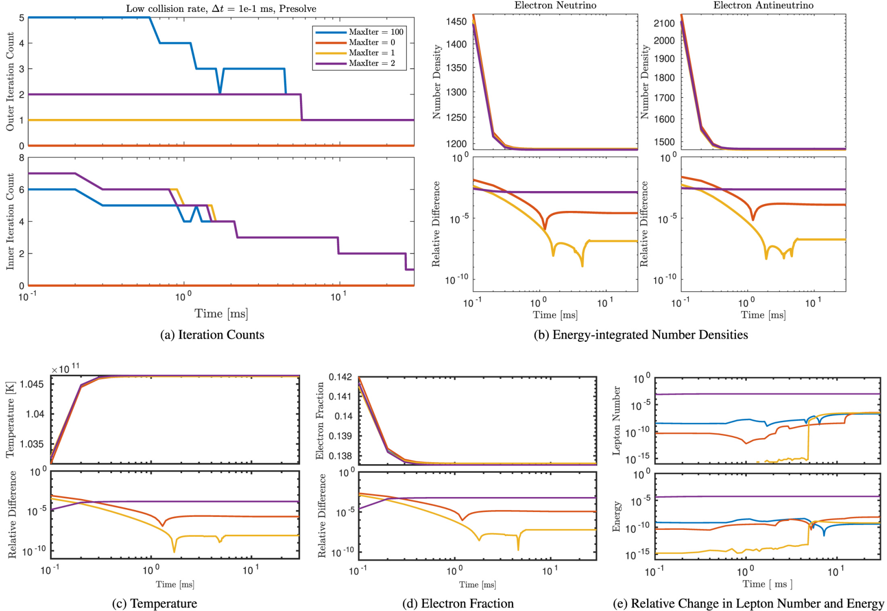
Figure 9. from A DG-IMEX Method for Two-moment Neutrino Transport: Nonlinear Solvers for Neutrino–Matter Coupling null 2021 APJS 253 52 doi:10.3847/1538-4365/abe2a8 https://dx.doi.org/10.3847/1538-4365/abe2a8 © 2021. The American Astronomical Society. All rights reserved.
