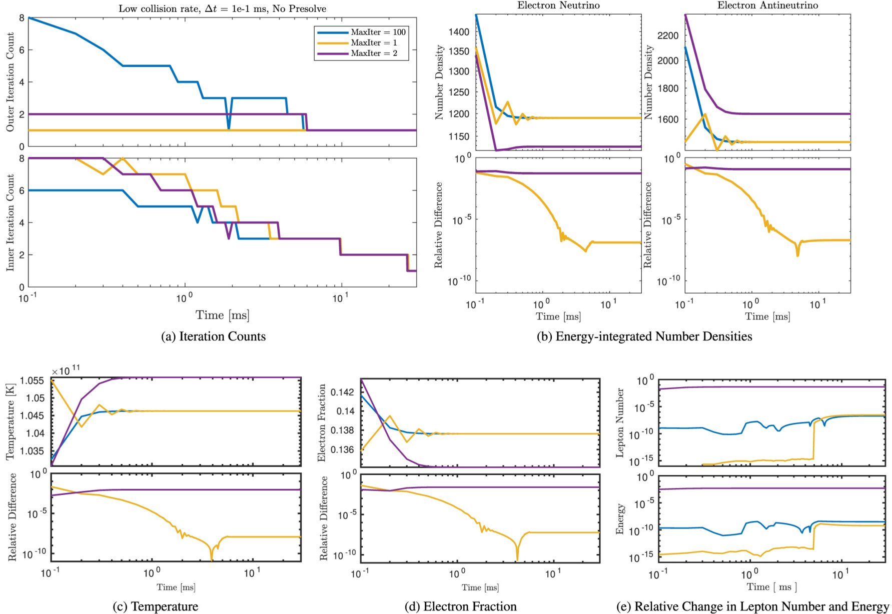
Figure 8. from A DG-IMEX Method for Two-moment Neutrino Transport: Nonlinear Solvers for Neutrino–Matter Coupling null 2021 APJS 253 52 doi:10.3847/1538-4365/abe2a8 https://dx.doi.org/10.3847/1538-4365/abe2a8 © 2021. The American Astronomical Society. All rights reserved.
