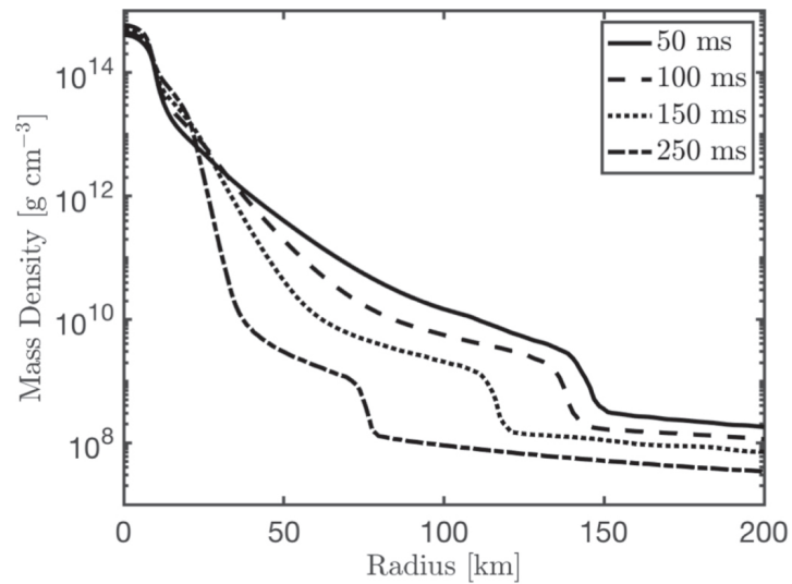
(a) Mass Density
