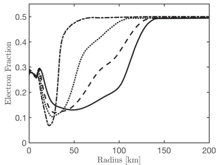
(c) Electron Fraction
