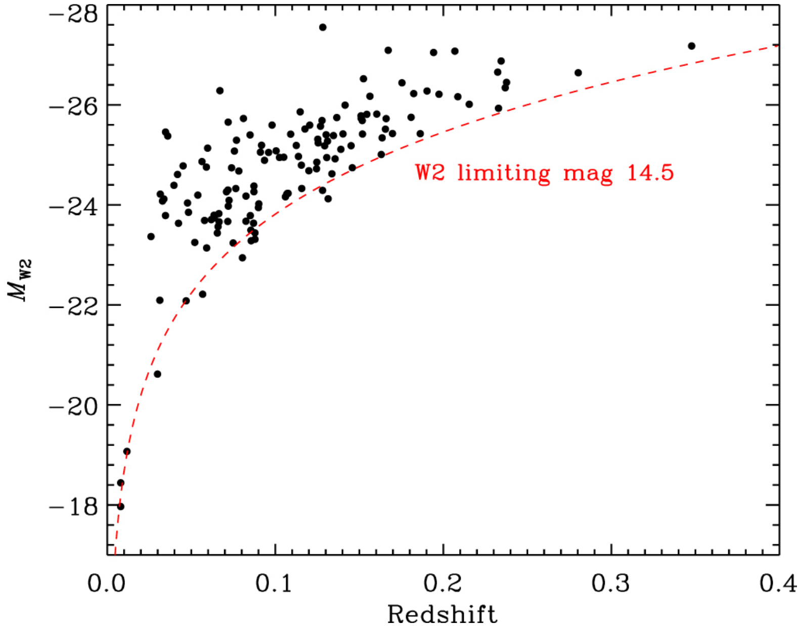
Figure 9. from Mid-infrared Outbursts in Nearby Galaxies (MIRONG). I. Sample Selection and Characterization null 2021 APJS 252 32 doi:10.3847/1538-4365/abd1dc https://dx.doi.org/10.3847/1538-4365/abd1dc © 2021. The American Astronomical Society. All rights reserved.
