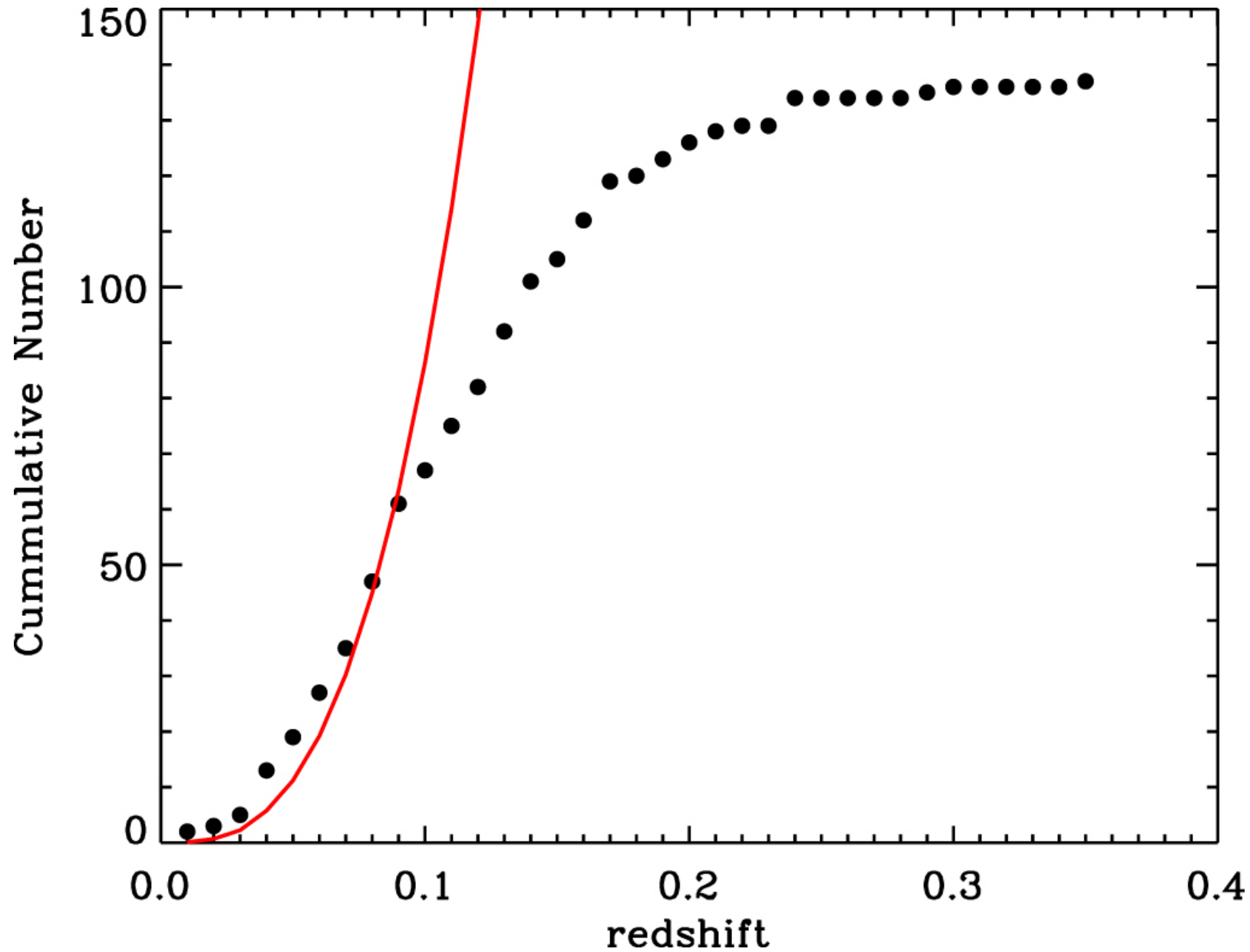
Figure 8. from Mid-infrared Outbursts in Nearby Galaxies (MIRONG). I. Sample Selection and Characterization null 2021 APJS 252 32 doi:10.3847/1538-4365/abd1dc https://dx.doi.org/10.3847/1538-4365/abd1dc © 2021. The American Astronomical Society. All rights reserved.
