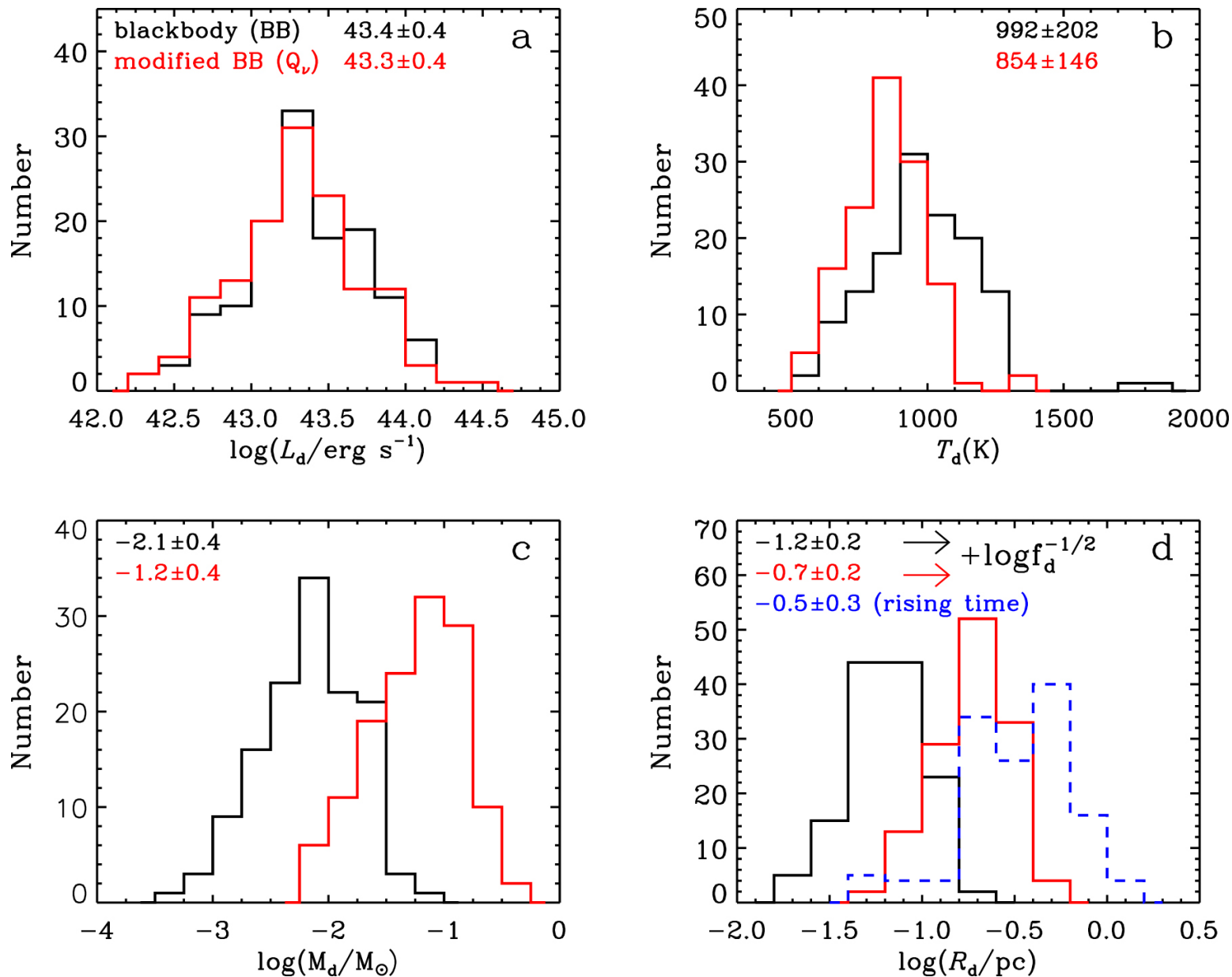
Figure 7. from Mid-infrared Outbursts in Nearby Galaxies (MIRONG). I. Sample Selection and Characterization null 2021 APJS 252 32 doi:10.3847/1538-4365/abd1dc https://dx.doi.org/10.3847/1538-4365/abd1dc
