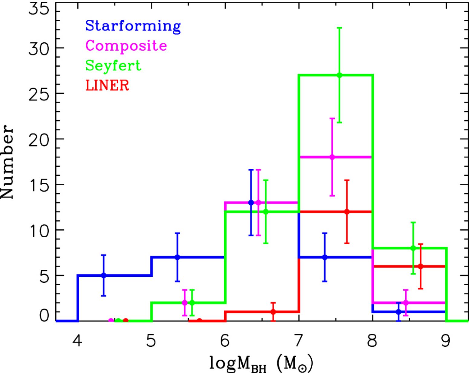
Figure 18. from Mid-infrared Outbursts in Nearby Galaxies (MIRONG). I. Sample Selection and Characterization null 2021 APJS 252 32 doi:10.3847/1538-4365/abd1dc https://dx.doi.org/10.3847/1538-4365/abd1dc © 2021. The American Astronomical Society. All rights reserved.
