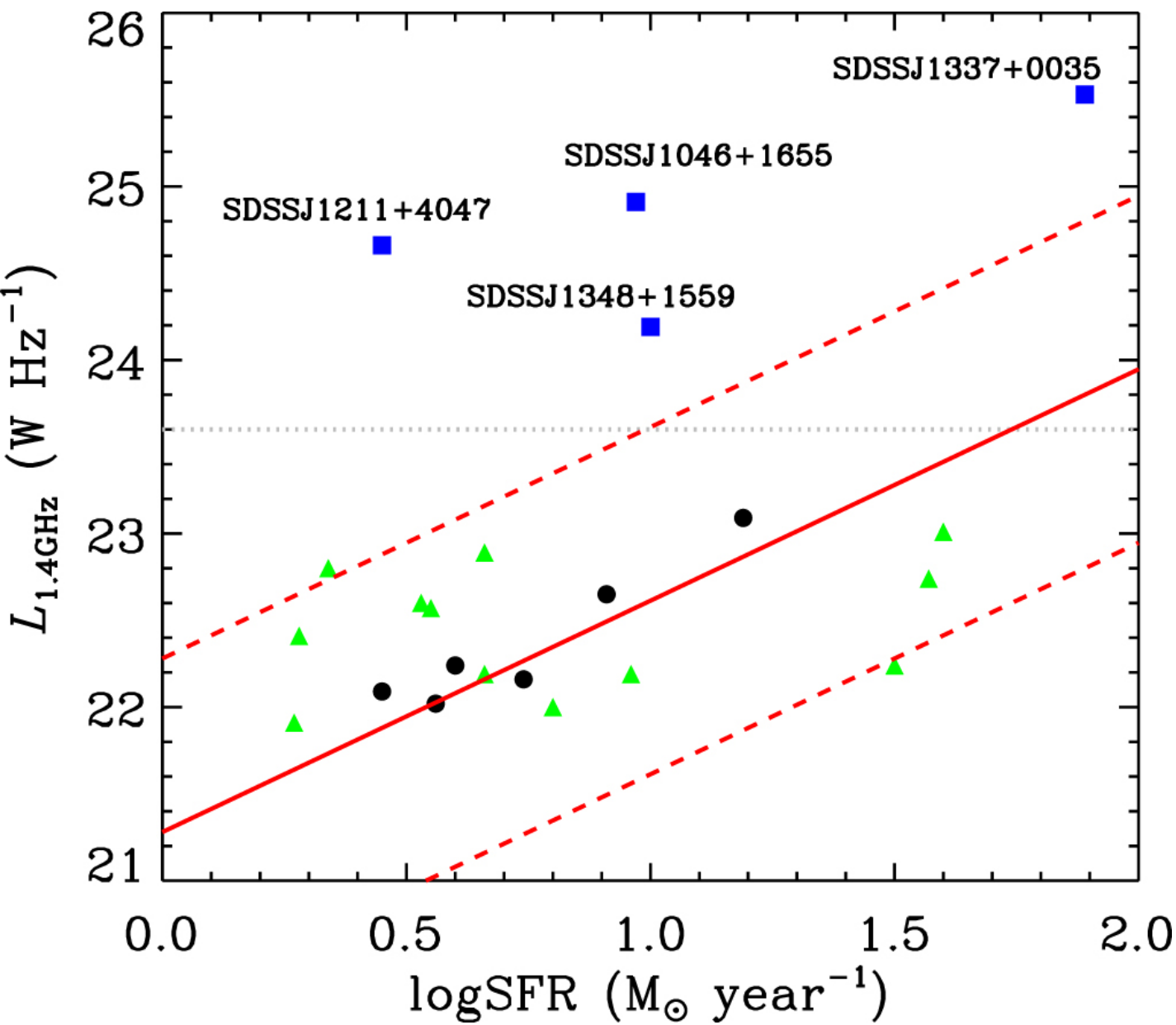
Figure 17. from Mid-infrared Outbursts in Nearby Galaxies (MIRONG). I. Sample Selection and Characterization null 2021 APJS 252 32 doi:10.3847/1538-4365/abd1dc https://dx.doi.org/10.3847/1538-4365/abd1dc © 2021. The American Astronomical Society. All rights reserved.
