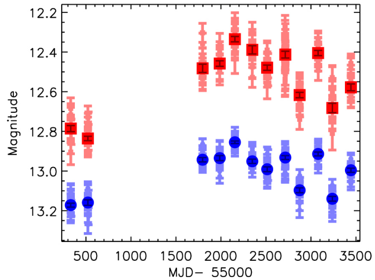
SDSSJ1046+3351
