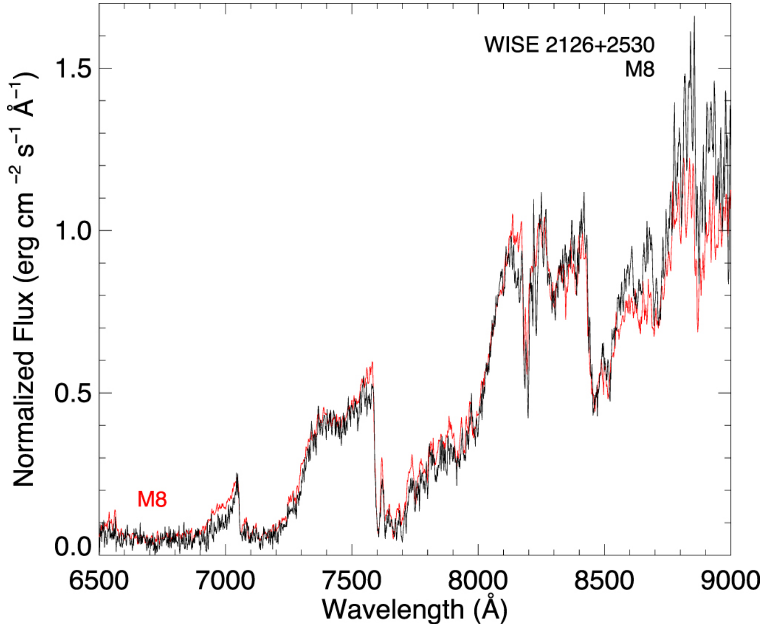
Figure 9. from The Field Substellar Mass Function Based on the Full-sky 20 pc Census of 525 L, T, and Y Dwarfs null 2021 APJS 253 7 doi:10.3847/1538-4365/abd107 https://dx.doi.org/10.3847/1538-4365/abd107 © 2021. The American Astronomical Society. All rights reserved.
