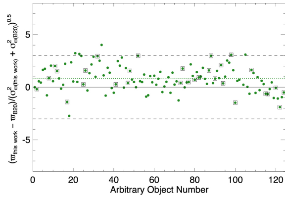
Figure 8. from The Field Substellar Mass Function Based on the Full-sky 20 pc Census of 525 L, T, and Y Dwarfs null 2021 APJS 253 7 doi:10.3847/1538-4365/abd107 https://dx.doi.org/10.3847/1538-4365/abd107
