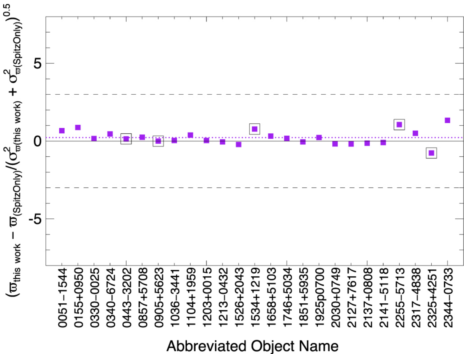
Figure 7. from The Field Substellar Mass Function Based on the Full-sky 20 pc Census of 525 L, T, and Y Dwarfs null 2021 APJS 253 7 doi:10.3847/1538-4365/abd107 https://dx.doi.org/10.3847/1538-4365/abd107 © 2021. The American Astronomical Society. All rights reserved.
