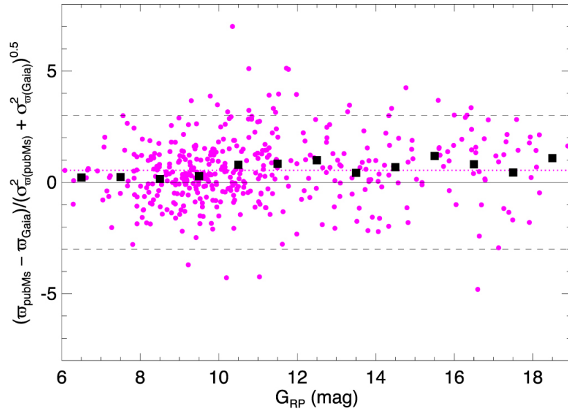
Figure 6. from The Field Substellar Mass Function Based on the Full-sky 20 pc Census of 525 L, T, and Y Dwarfs null 2021 APJS 253 7 doi:10.3847/1538-4365/abd107 https://dx.doi.org/10.3847/1538-4365/abd107 © 2021. The American Astronomical Society. All rights reserved.
