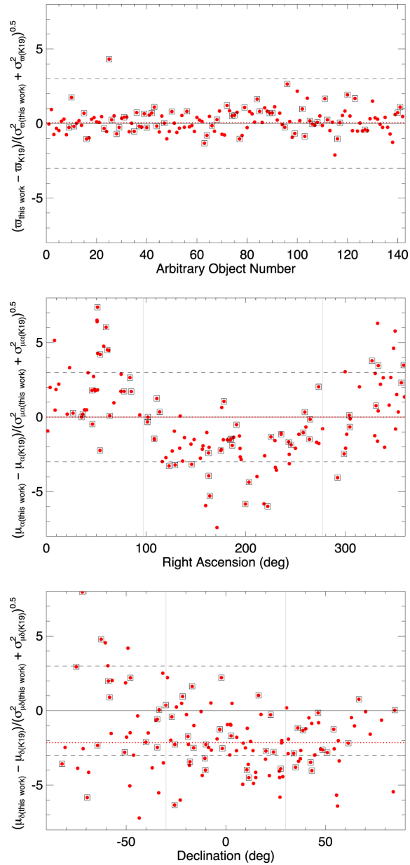
Figure 4. from The Field Substellar Mass Function Based on the Full-sky 20 pc Census of 525 L, T, and Y Dwarfs null 2021 APJS 253 7 doi:10.3847/1538-4365/abd107 https://dx.doi.org/10.3847/1538-4365/abd107
