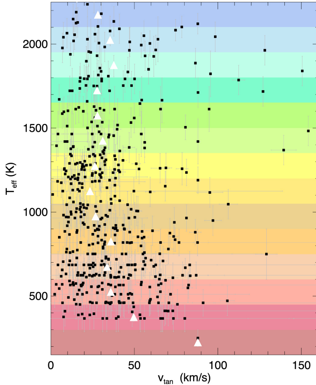
Figure 33. from The Field Substellar Mass Function Based on the Full-sky 20 pc Census of 525 L, T, and Y Dwarfs null 2021 APJS 253 7 doi:10.3847/1538-4365/abd107 https://dx.doi.org/10.3847/1538-4365/abd107 © 2021. The American Astronomical Society. All rights reserved.
