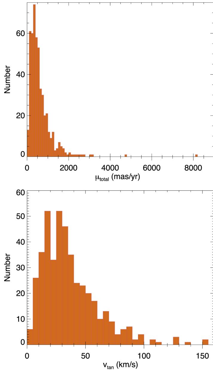
Figure 32. from The Field Substellar Mass Function Based on the Full-sky 20 pc Census of 525 L, T, and Y Dwarfs null 2021 APJS 253 7 doi:10.3847/1538-4365/abd107 https://dx.doi.org/10.3847/1538-4365/abd107 © 2021. The American Astronomical Society. All rights reserved.
