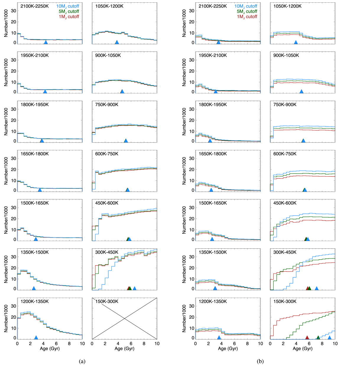
Figure 31. from The Field Substellar Mass Function Based on the Full-sky 20 pc Census of 525 L, T, and Y Dwarfs null 2021 APJS 253 7 doi:10.3847/1538-4365/abd107 https://dx.doi.org/10.3847/1538-4365/abd107
