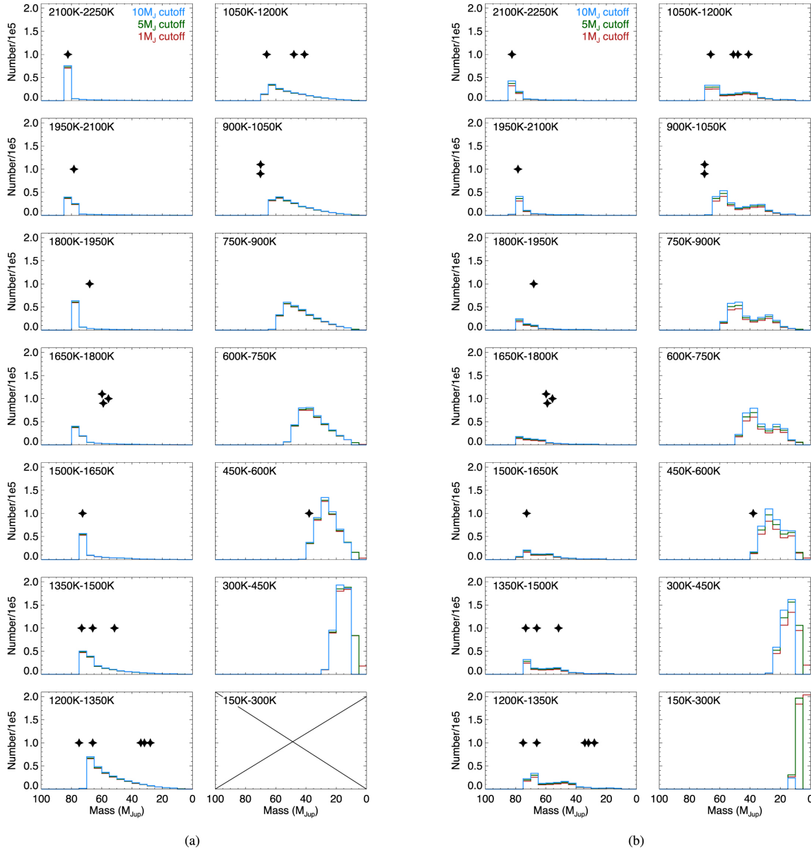
Figure 30. from The Field Substellar Mass Function Based on the Full-sky 20 pc Census of 525 L, T, and Y Dwarfs null 2021 APJS 253 7 doi:10.3847/1538-4365/abd107 https://dx.doi.org/10.3847/1538-4365/abd107 © 2021. The American Astronomical Society. All rights reserved.
